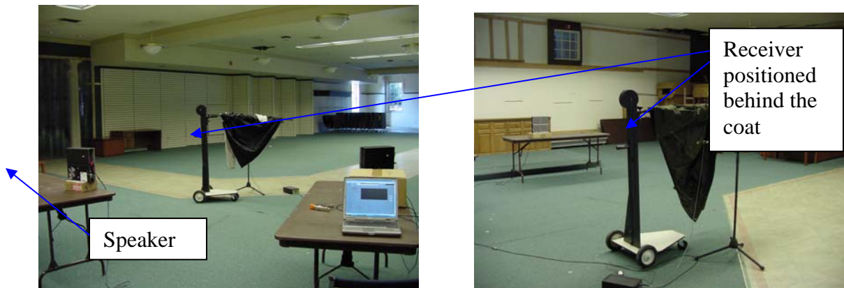
Figure A1: Experimental set-up for show that non-linear acoustic approach has the capability to see through thick clothing
