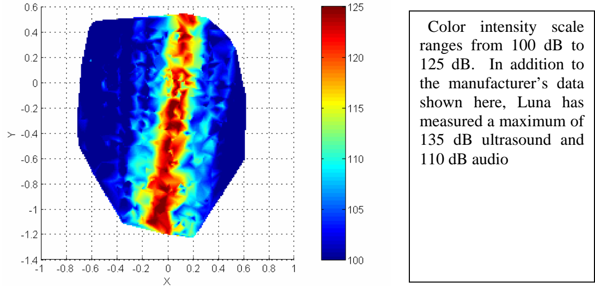
Figure 13: A plot of calibration data for ultrasonic sound pressure amplitudes with the xy origin at 15 ft.
