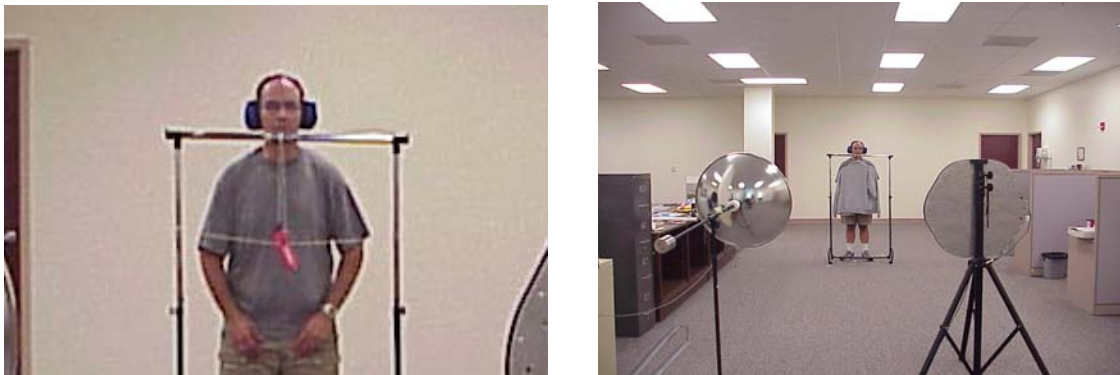
Figure 22: Pictures of experimental set-up for detecting signatures through thick clothing
