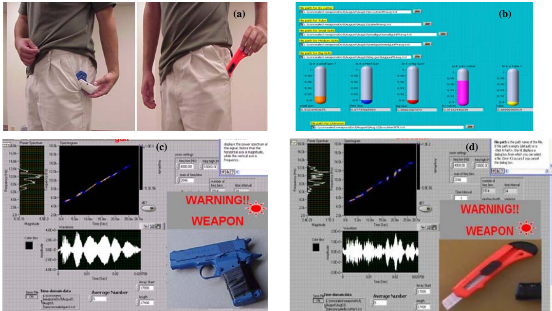
Figure 1: Long range detection of concealed weapons for street systems from 15 feet.
