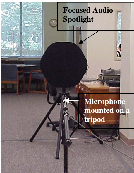
Figure 12: Experimental set-up showing the beam characterization at 15 feet for a focused audio spotlight.
