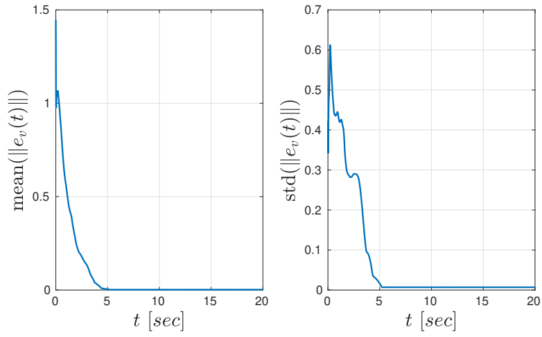
Figure 4: Mean (left) and standard deviation (right) of e_v(t) for the proposed control policy.
