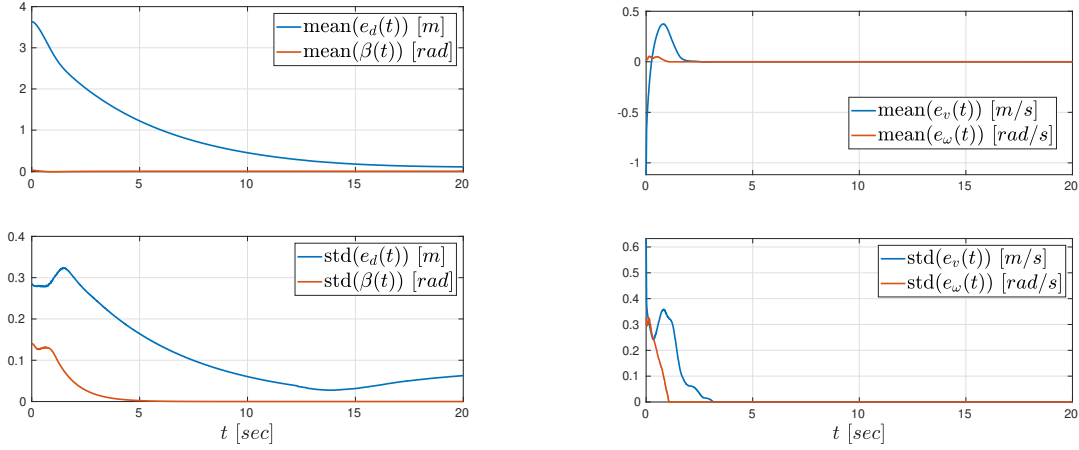
(a) Mean (top) and standard deviation (bottom) of e_d(t) , \beta(t) for the unicycle system. (b) Mean (top) and standard deviation (bottom) of e_v(t) and e_\omega(t) for the unicycle system.
