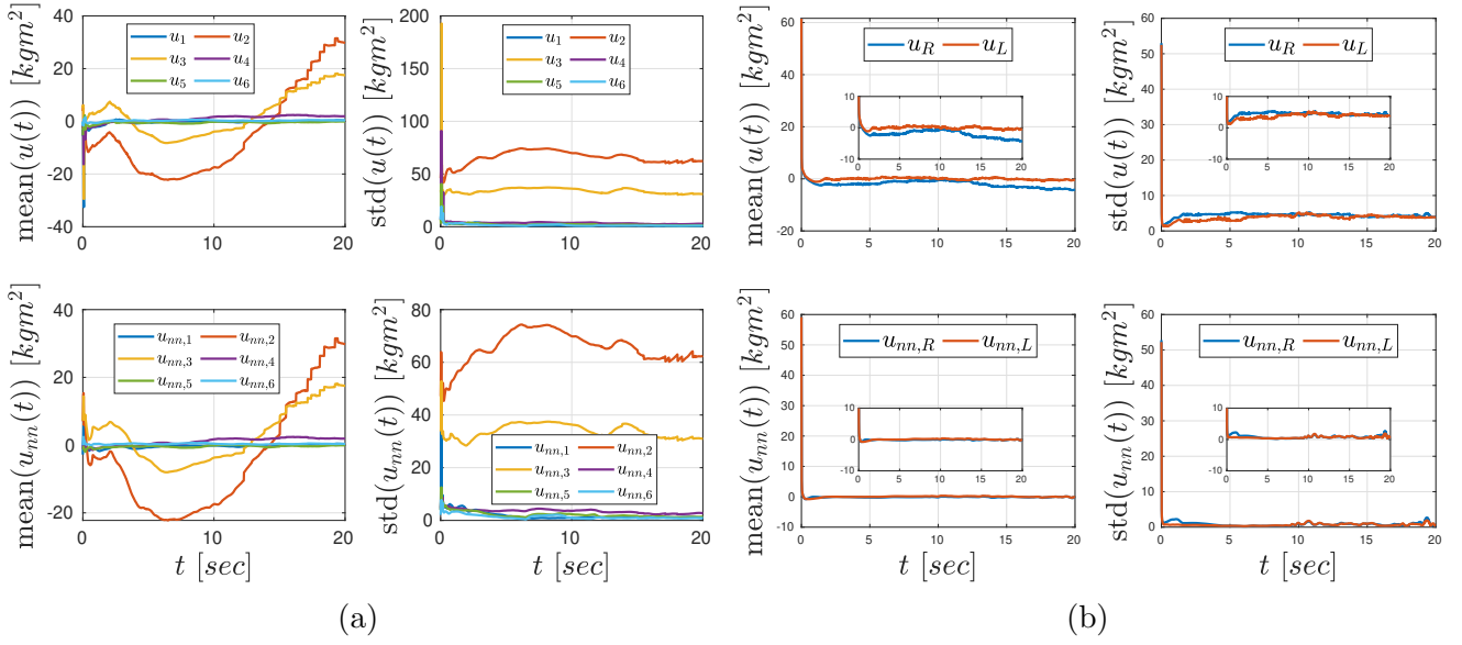
Figure 7: (a): Mean (left) and standard deviation (right) of u(t) (top) and u_{nn}(t) (bottom) for the proposed control policy and the robotic-manipulator system. (b): Mean and standard deviation (right) of u(t) (top) and u_{nn}(t) (bottom) for the proposed control policy and the unicycle system.
