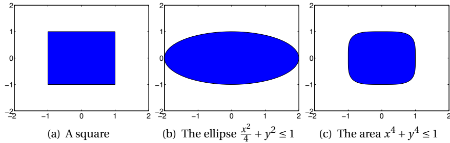
Figure 2.1: Examples of some convex sets.
