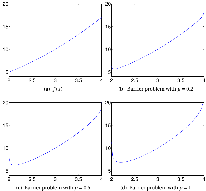
Figure 6.1: The function from Example 6.3 and some of its barrier functions.
