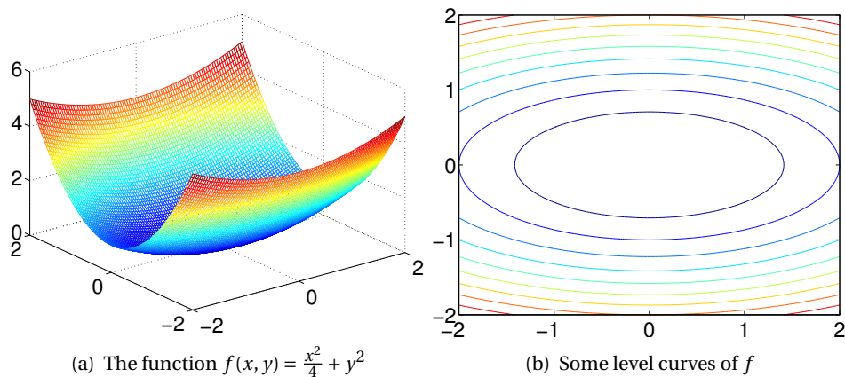
Figure 2.2: A function and its level curves.
