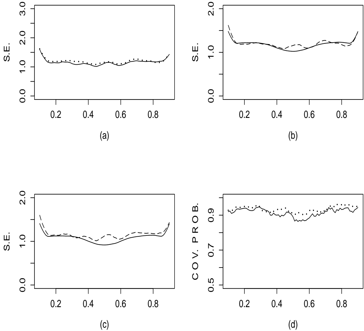
Figure 2: (a) Comparison of the empirical SEs of the working independent kernel estimate \widehat{\theta}_I^{(1)}(z) and the weighted kernel estimates \widehat{\theta}_W^{(1)}(z) : \cdots \widehat{\theta}_I^{(1)}(z) , — \widehat{\theta}_W^{(1)}(z) . (b) Comparison of the empirical and sandwich SE estimates of the working independence kernel estimator \widehat{\theta}_I^{(1)}(z) : \cdots Estimated sandwich standard error; — the empirical standard error. (c) Comparison of the empirical and sandwich SEs of the weighted kernel estimator \widehat{\theta}_W^{(1)}(z) : \cdots the estimated sandwich standard error; — the empirical standard error. (d) Empirical coverage probabilities of the 95% estimated point-wise confidence intervals: \cdots \theta_I^{(1)}(z) ; — \theta_W^{(1)}(z) . The bandwidth was set as h = 0.15 .
