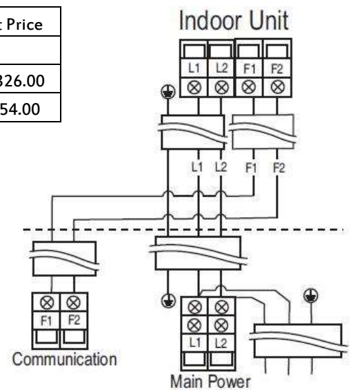
Wiring diagram
