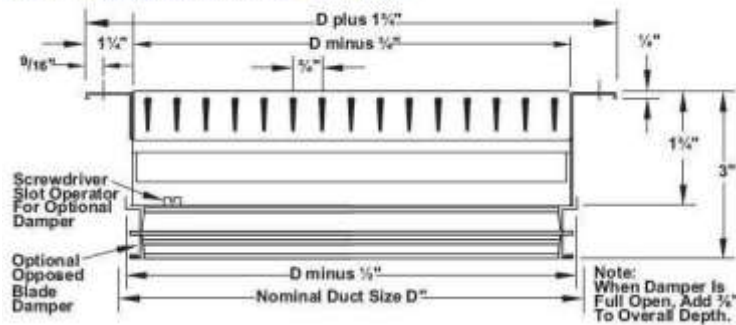
Double Deflection Models 300RL/RS - Border Type 1
