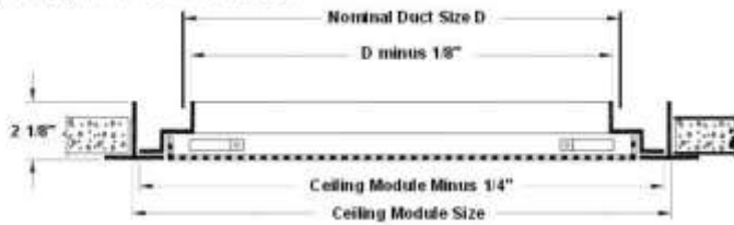
Border Type 3 (Lay-In when D=Module size -2)
