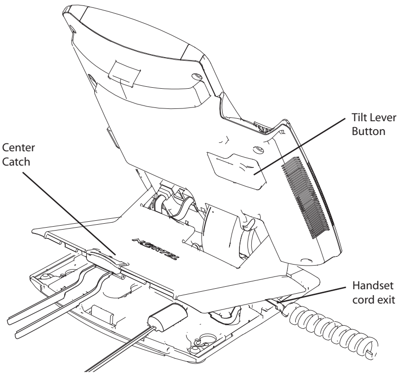
Figure 5: Remove the stand cover
