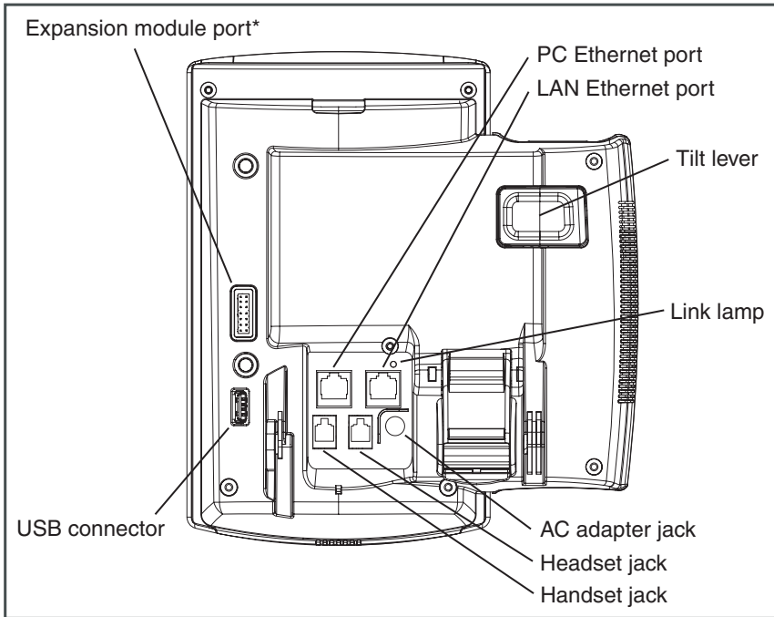
Figure 4: IP Phone 1120E connections
