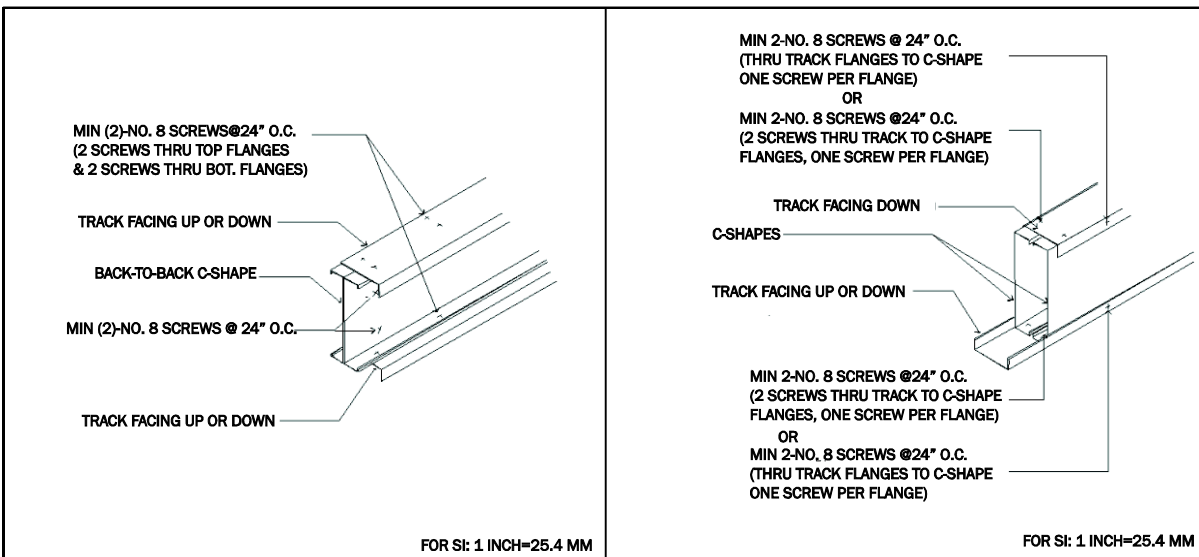
Figure C3.4.4-1 Back-to-Back Header
