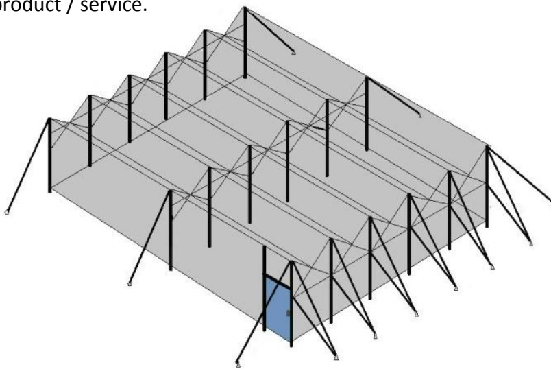
TWO SLOPE SHADENET COVERED STRUCTURE STEEL WIRE WITH G.I. PIPE FOR VINEYARDS AND ORCHARDS
