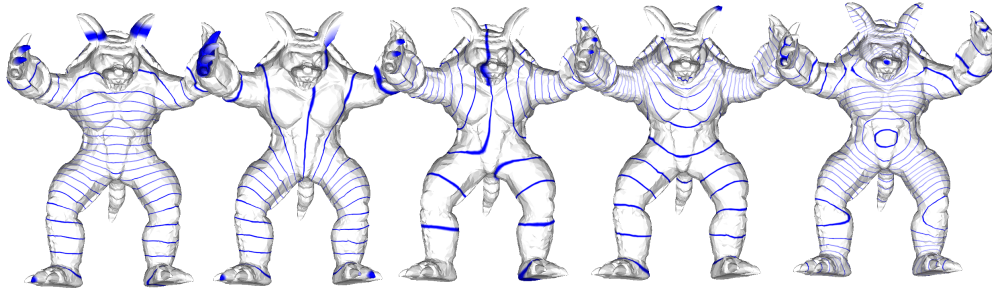
Picture from the article Laplace-Beltrami eigenfunctions towards an algorithm that “understands” the geometry .
