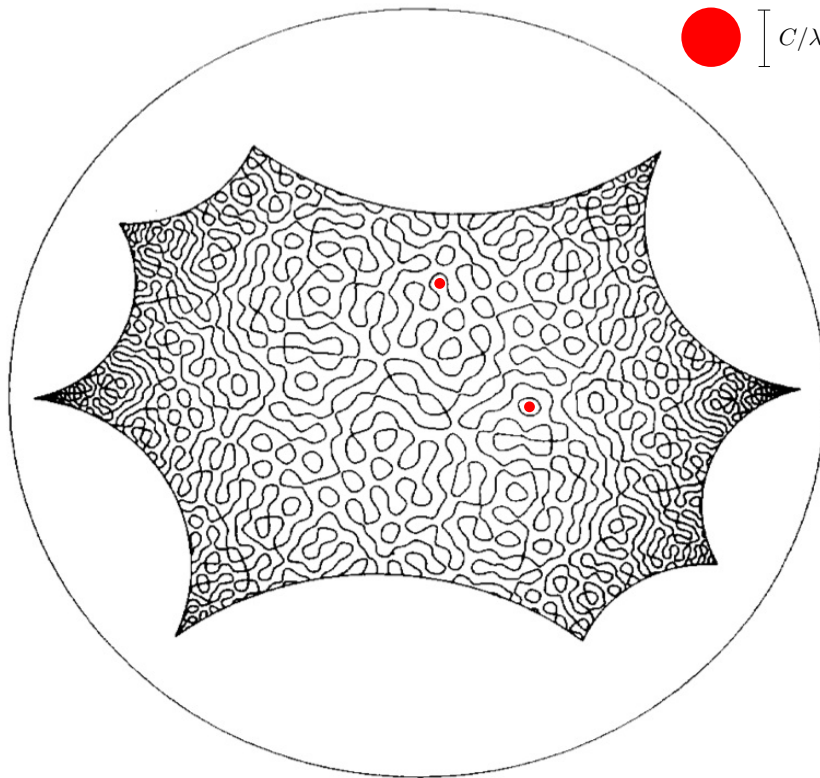
Figure: Nodal set of a bitorus
