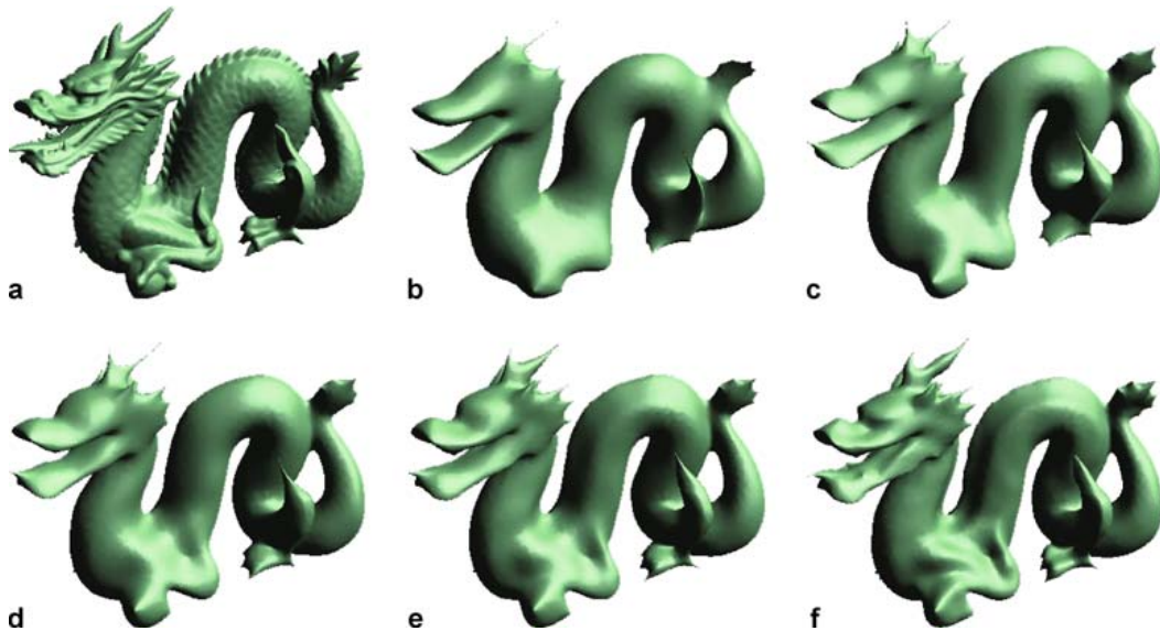
a. M = \text{Dragon} . b-f. reconstructed manifold using N = 100, 200, 300, 500 and 900 eigenfunctions respectively. Picture from paper Spectral mesh deformation .
