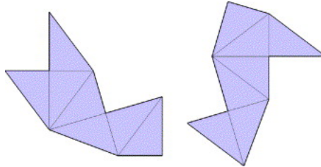
Figure: Two domains with the same eigenvalues
