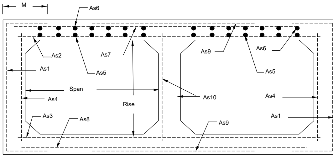
Typical Reinforcement Layout
