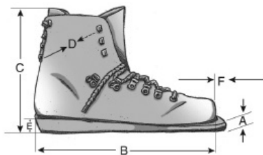
FIGURE 4 SHOOTING SHOES
