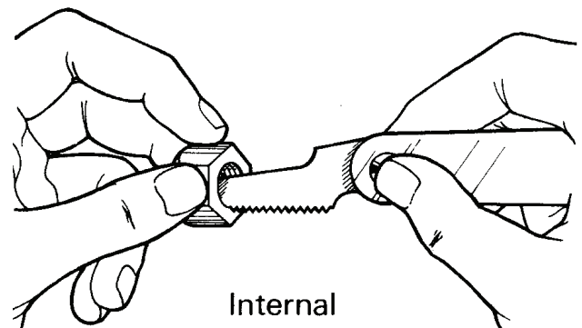
USE OF SCREW PITCH GAUGES
