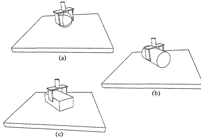
Fig. 1. Constrained end-effector freedom of motion. (a) Five degrees of freedom. (b) Four degrees of freedom. (c) Three degrees of freedom.
