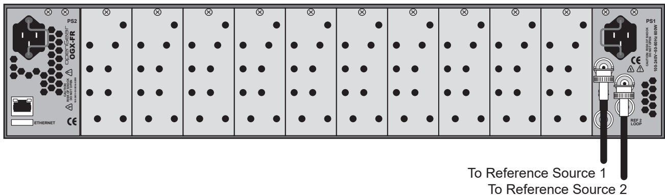
Figure 6.1 OGX-FR — Reference Input Cabling
