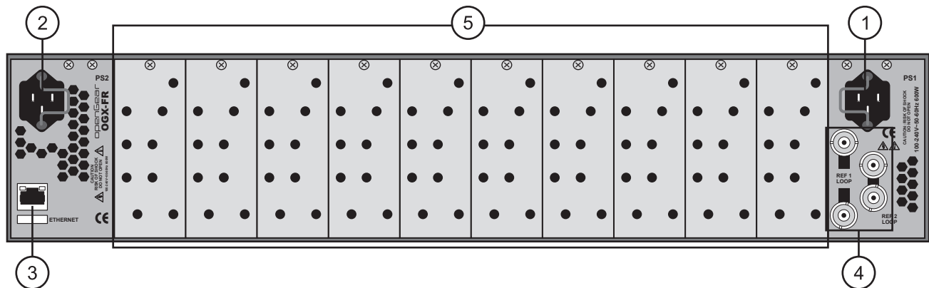
Figure 3.3 OGX-FR — Rear Panel
