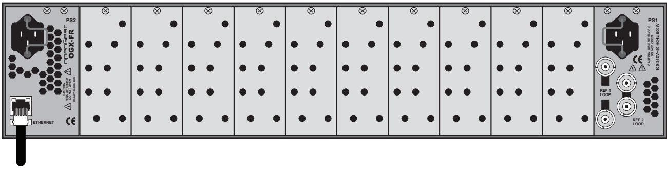
Figure 5.1 OGX-FR Frame — Ethernet Cabling
