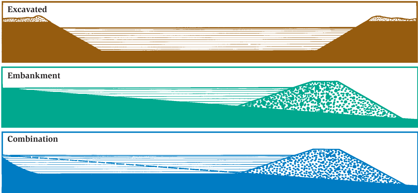
Figure 1.2. Pond types: excavated, embankment, combination.
