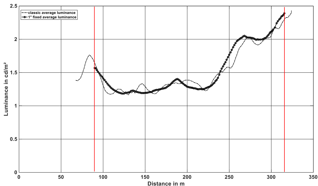
Figure 6 – Comparison of average luminance with classic measurements and with 1^\circ fixed measurements
