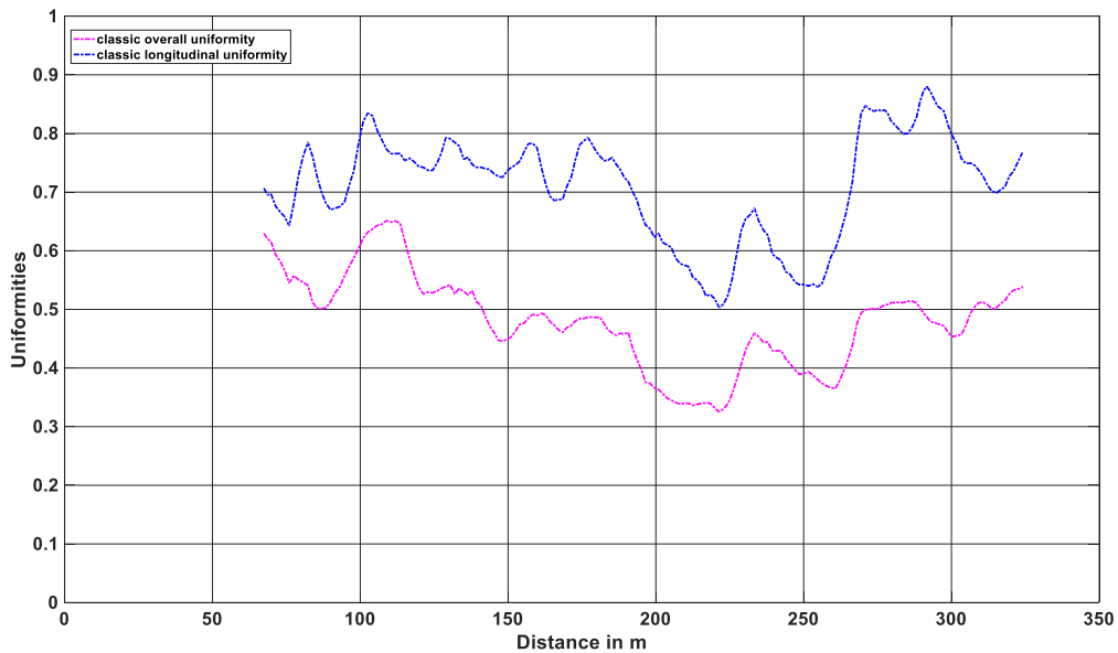
Figure 5 – Continuous uniformities measurements for classic methodology
