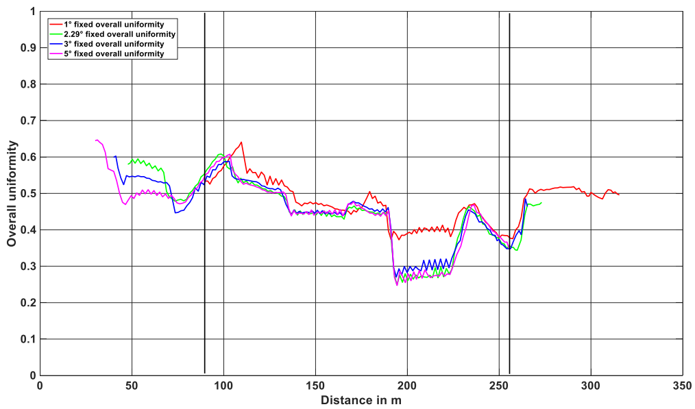
Figure 11 – Comparison of overall uniformity for 1° (in red), 2.29° (in green), 3° (in blue) and 5° (in pink) fixed measurements
