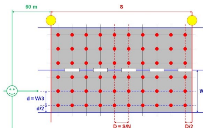
Figure 1 – Measurement grid points in road lighting
