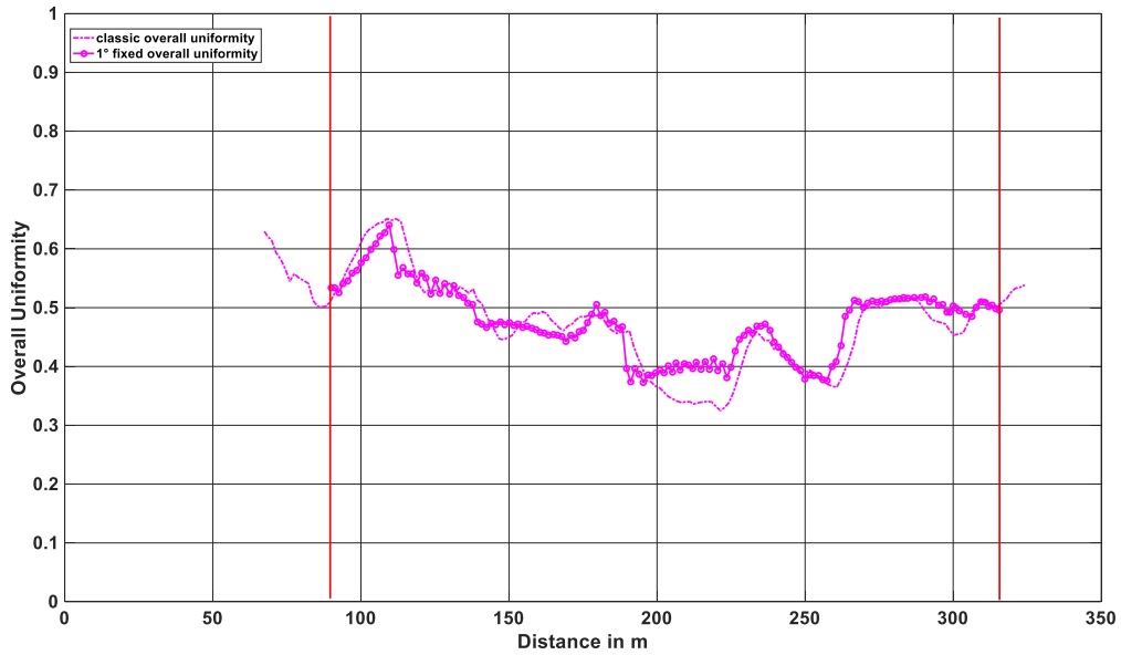
Figure 7 – Comparison of overall uniformity with classic measurements and with 1° fixed measurements
