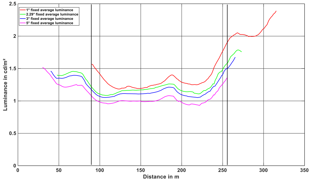
Figure 10 – Comparison of average luminance for 1° (in red), 2.29° (in green), 3° (in blue) and 5° (in pink) fixed measurements
