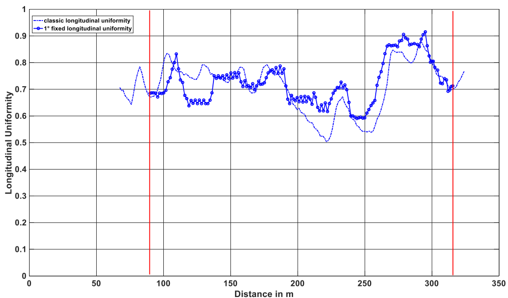
Figure 8 – Comparison of longitudinal uniformity with classic measurements and with 1° fixed measurements
