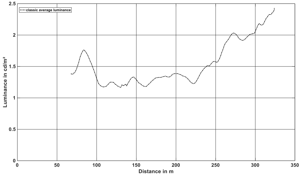
Figure 4 – Continuous average luminance measurements for classic methodology
