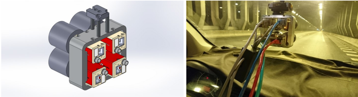
Figure 2 – HDR-ILMD developed by Cerema
