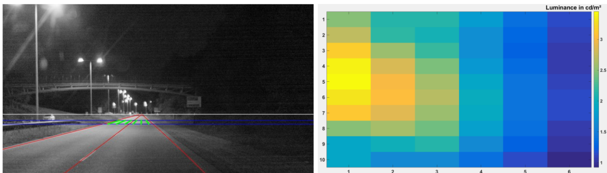
Figure 3 – Measurement grid points positioning (left) and luminances at the grid points (right) – (Greffier, 2015)
