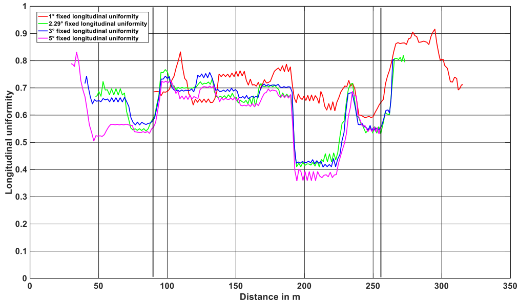
Figure 12 – Comparison of longitudinal uniformity for 1° (in red), 2.29° (in green), 3° (in blue) and 5° (in pink) fixed measurements
