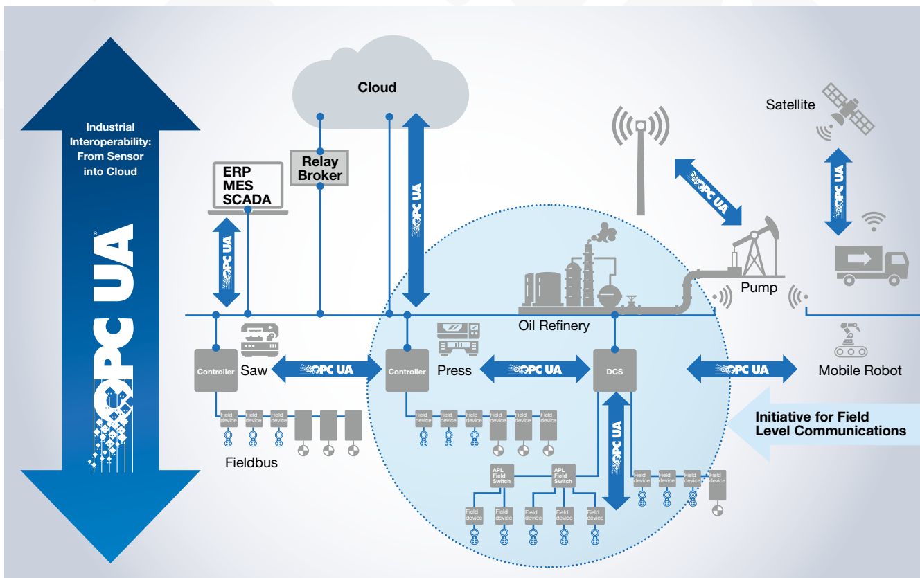
Figure 1: OPC UA use cases and scope of OPC Foundation's Field Level Communications Initiative
