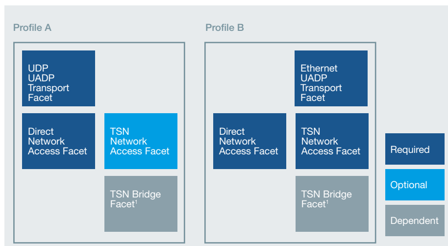
Figure 22: Structure of communications profiles
