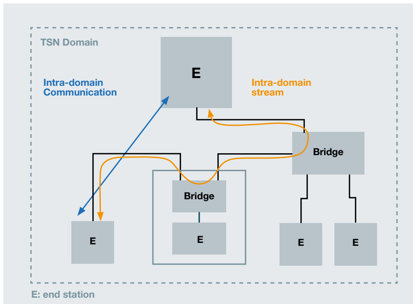
Figure 26: Intra-domain communication
