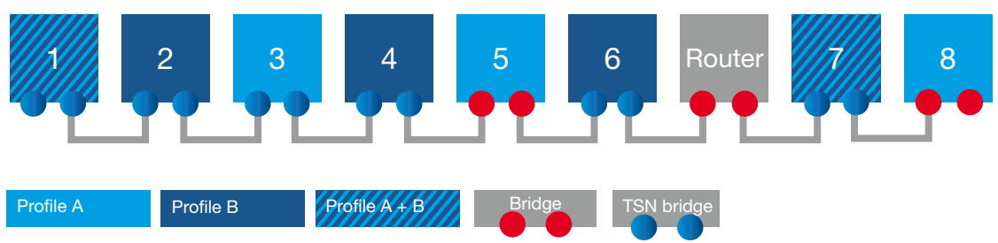
Figure 24: Topology to illustrate interoperability in a mixed Profile A/Profile B scenario
