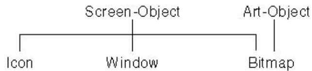
Figure 4-10. Multiple Inheritance
