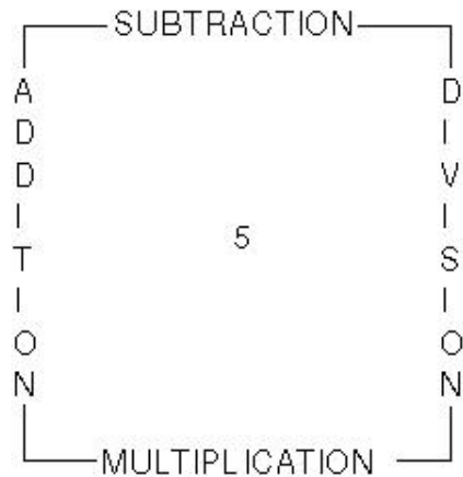
Figure 4-4. Encapsulated 5 Object
