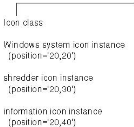
Figure 4-6. Icon Class
