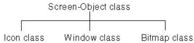
Figure 4-9. The Screen-Object Superclass
