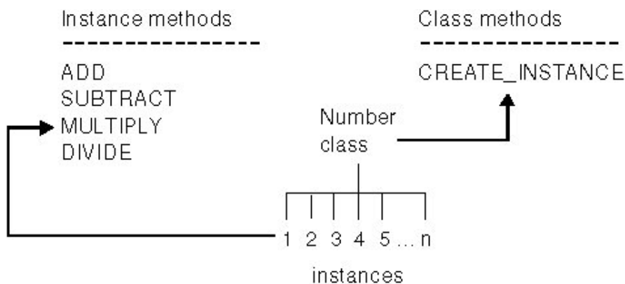
Figure 6-1. Instance Methods and Class Methods
