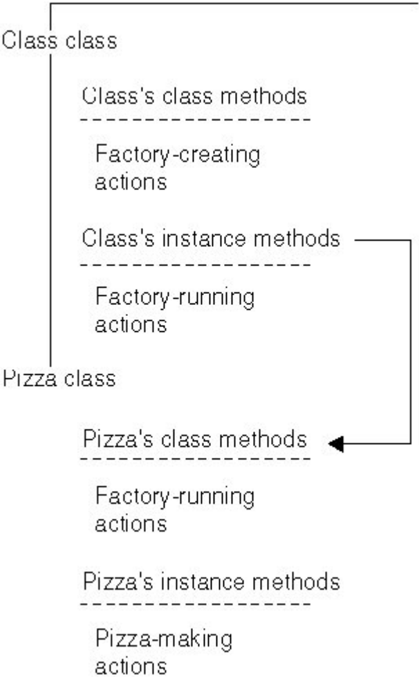
Figure 5-1. How Subclasses Inherit Instance Methods from the Class Class
