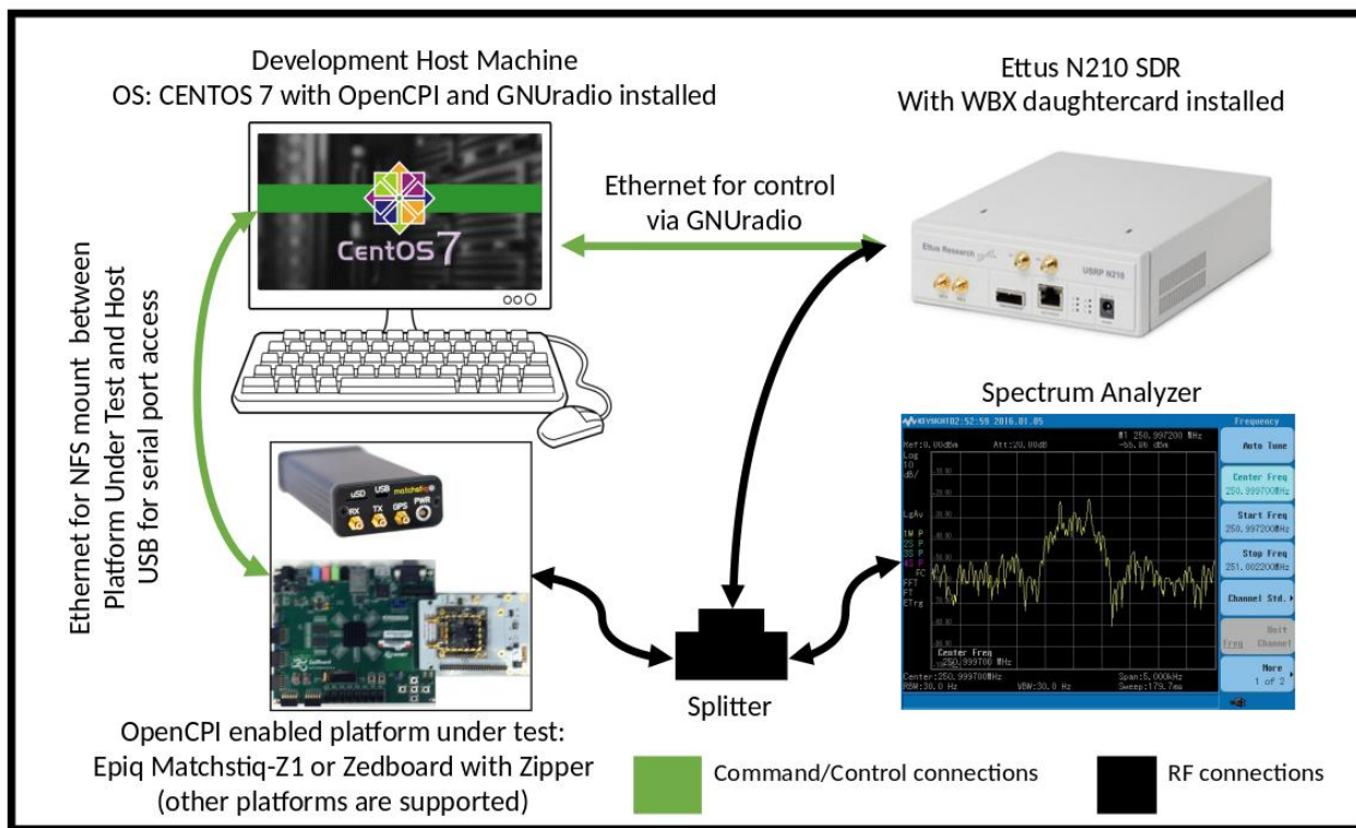
Figure 3: RX App Test Setup
