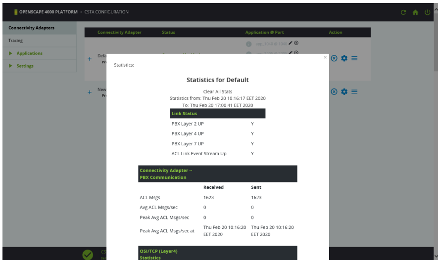
Figure 41: Statistics
