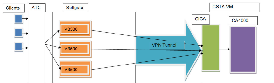
Figure 42: General architecture of the circuit connection
