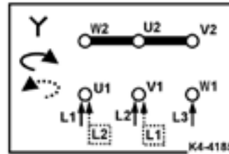
Star connection
