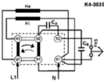
CA – start capacitor CB – run capacitor
