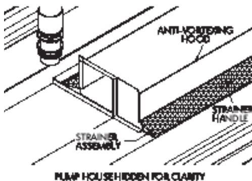
Figure 14 – PHC-D Strainer Assembly
