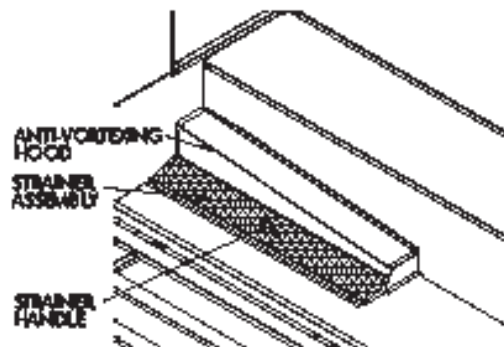
Figure 13 – PHC-S&L Strainer Assembly
