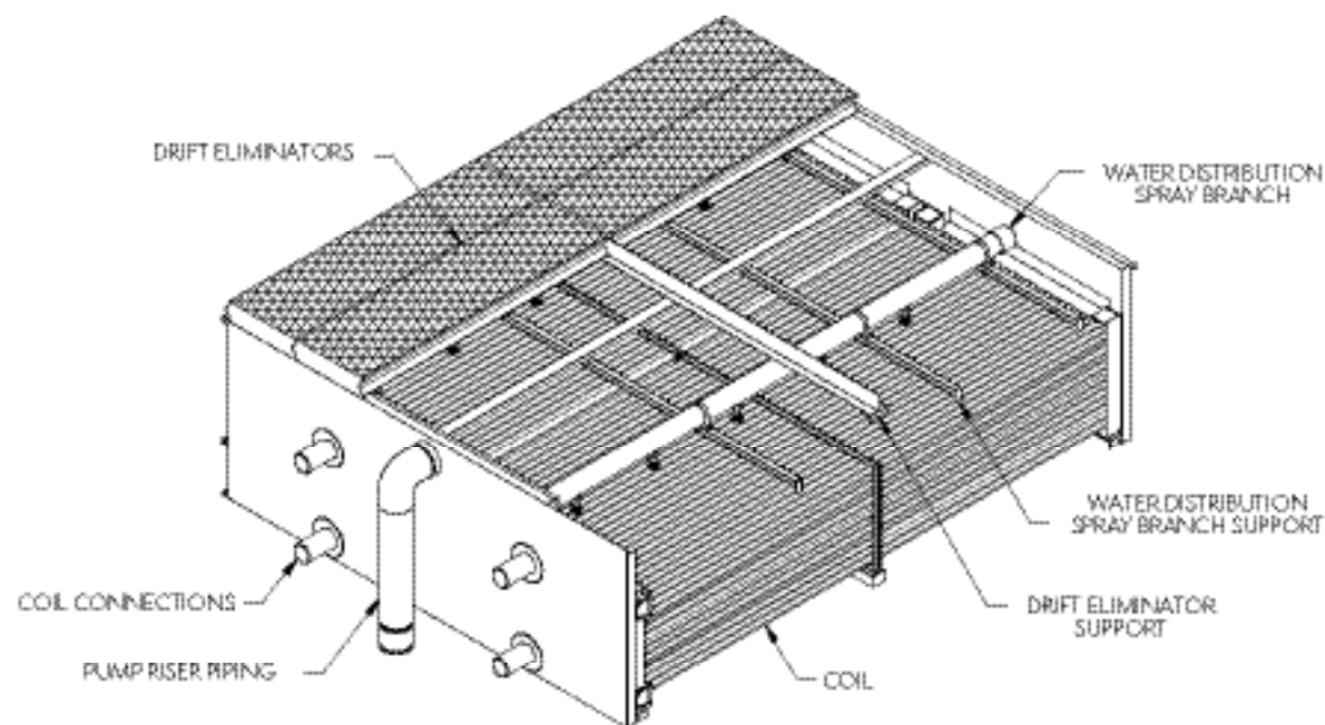
COIL CASING SECTION
