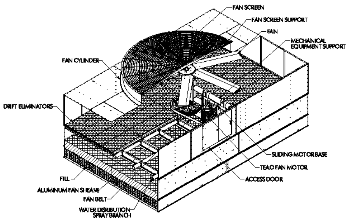
PAN SECTION
