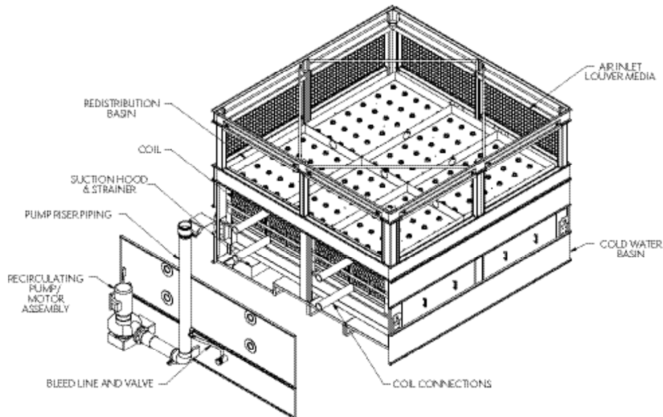
PAN SECTION
