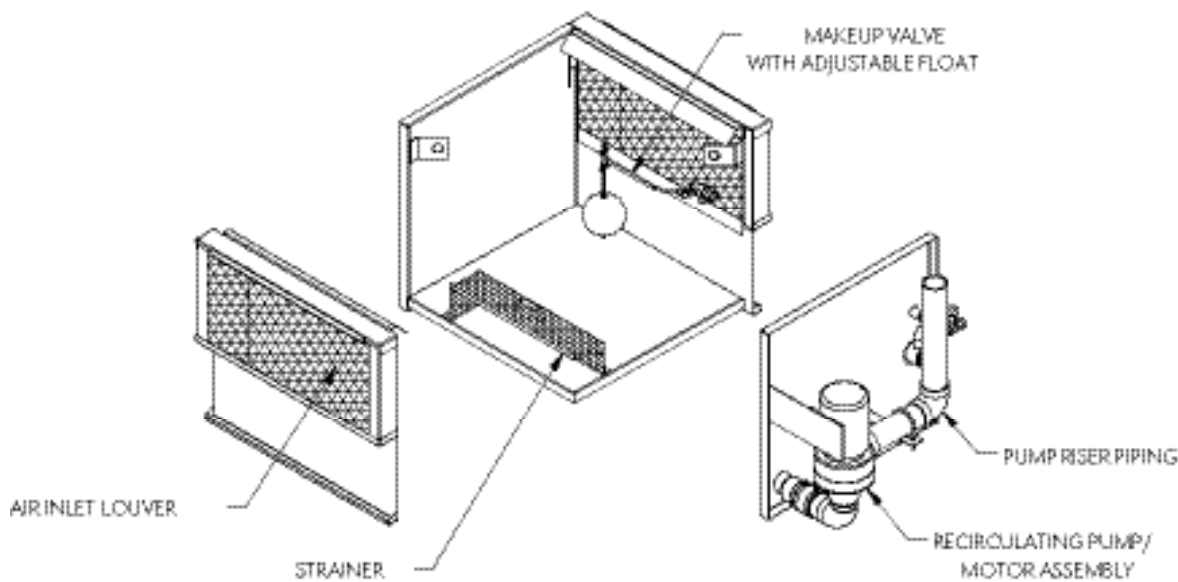
PAN SECTION
