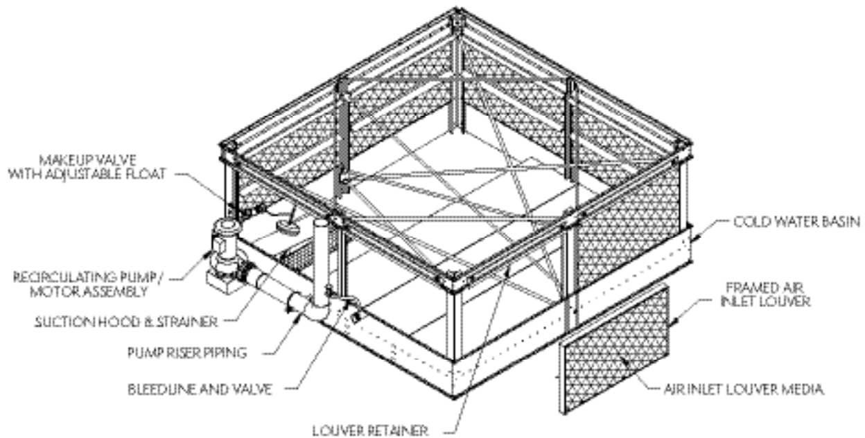
PAN SECTION
