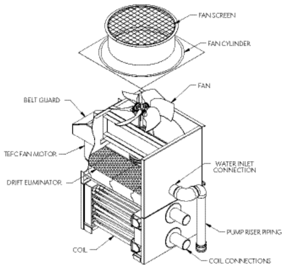
FAN & COIL CASING SECTION
