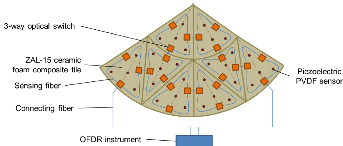
Schematic of Demonstrator (plan view)
