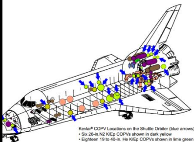
Figure 2. Kevlar®-epoxy (K/Ep) COPVs on shuttle.
