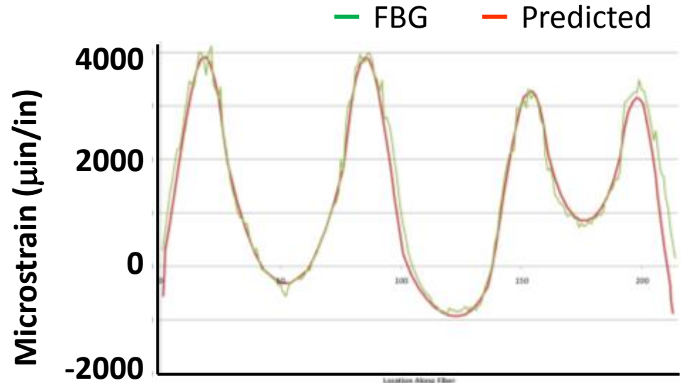
Inner Hatch FBG Strains, Max Pressure
