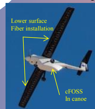
cFOSS v1.0 onboard APV-3
