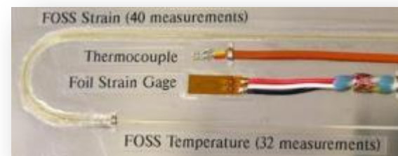
Metallic Coupon
