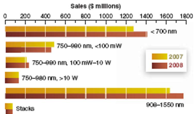
Figure 3. Worldwide diode-laser sales by type
