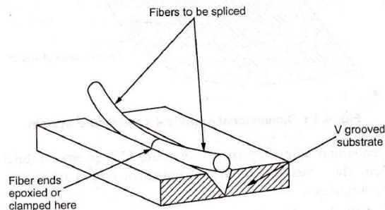
Fig. 4.2.2 V groove optical fiber splicing technique
