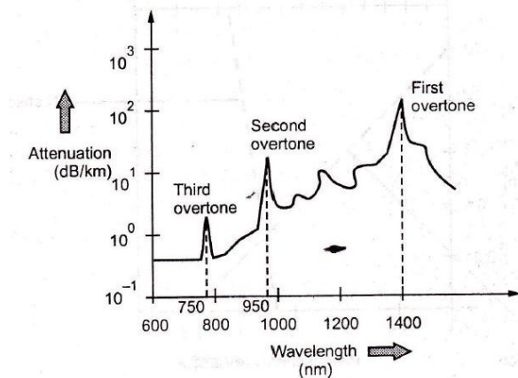
Fig. 2.2.2 Absorption spectra for OH group
