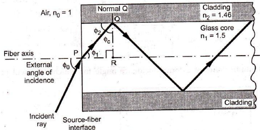
Fig. 1.6.8 Ray propagation by TIR
