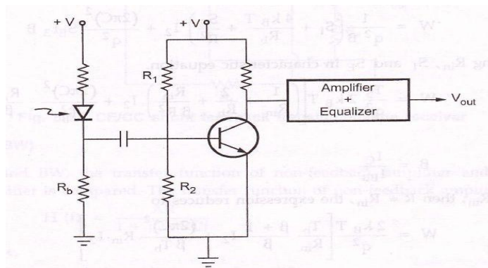
Fig. 5.1.6 High input impedance preamplifier using BJT
