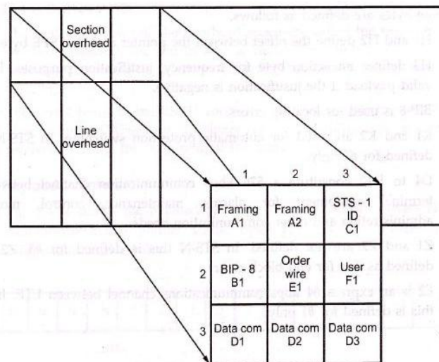
Fig. 8.4.12 STS-1 section overhead
