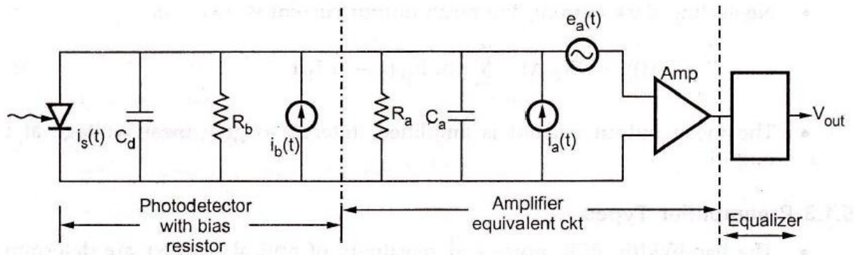
Fig. 5.1.3 High - input impedance preamplifier
