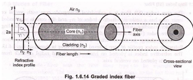
Fig. 1.6.14 Graded index fiber
