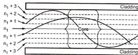
Fig. 1.6.19 Light trajectories in a graded index fiber
