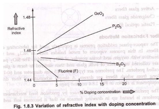
Fig. 1.8.3 Variation of refractive index with doping concentration
