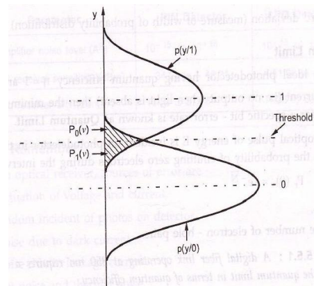
Fig. 5.5.1 Probability distribution of received 1 and 0
