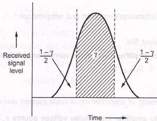
Fig. 5.2.1 Pulse spreading in adjacent time slot
