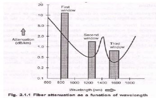
Fig. 2.1.1 Fiber attenuation as a function of wavelength
