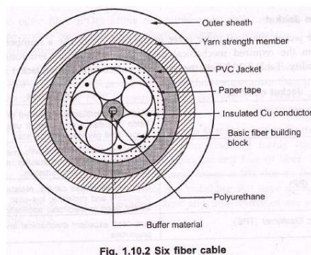
Fig. 1.10.2 Six fiber cable
