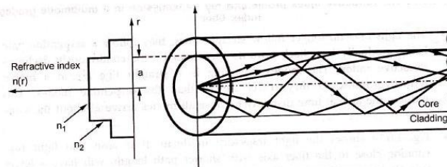
Fig. 1.6.17 TIR in multimode step index fiber
