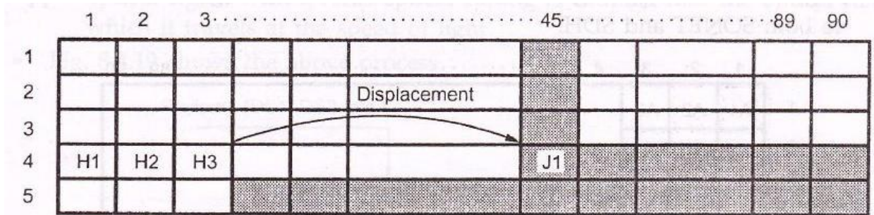
Fig. 8.4.16 STS-1 No frequency justification
