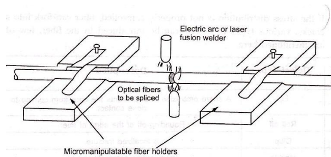
Fig. 4.2.1 Fusion splicing of optical fibers
