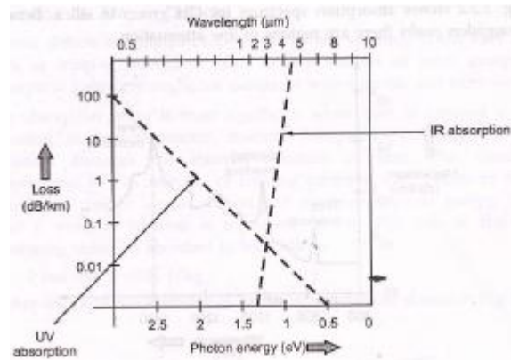
Fig. 2.2.3 Attenuation spectra for intrinsic loss
