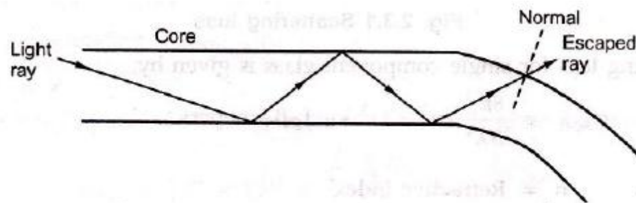
Fig. 2.4.1 Bending loss
