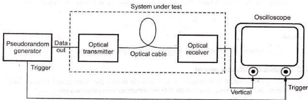
Fig. 8.7.3 Setup for Eye-diagram Measurement
