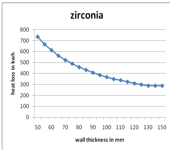
Graph 3: Effect of wall thickness on heat losses (Zirconia)
