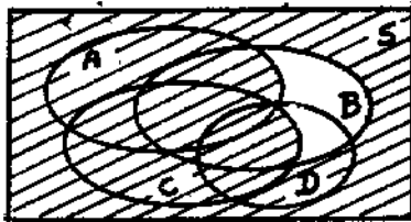
(c) (A \cup \bar{B}) \cup (C \cap D)
