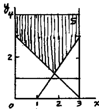
(b) C \cap B \cap \bar{A}
