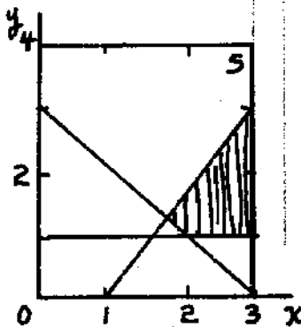
(c) (A \cup \bar{B}) \cup (C \cap D)
