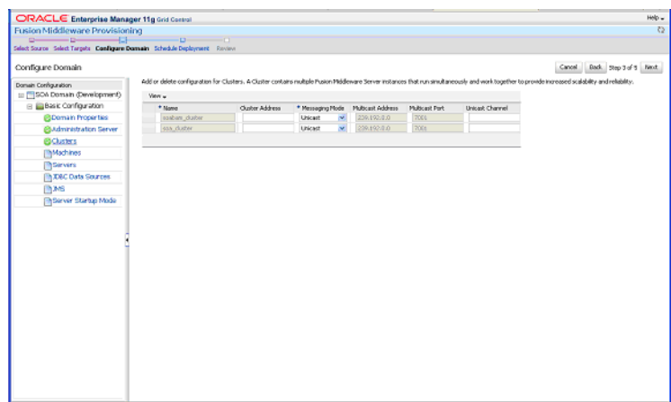
Figure 13–8 Clusters Page
