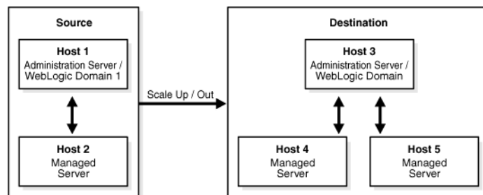
Figure 13–3 Fusion Middleware Domain Scale Up
