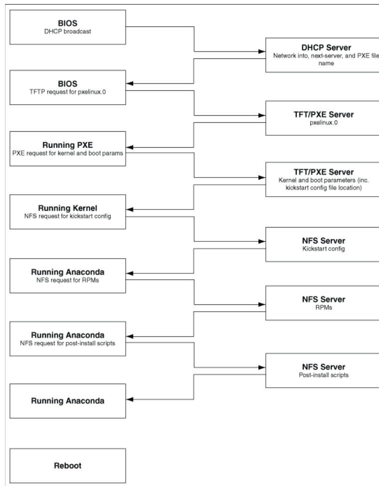
Figure 2–2 PXE Process
