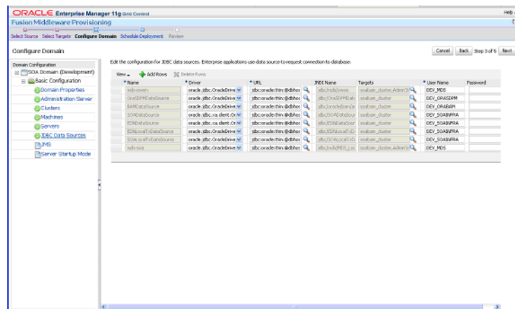
Figure 13–11 JDBC Data Sources Page
