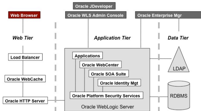
Figure 7: Oracle Platform Security Services
