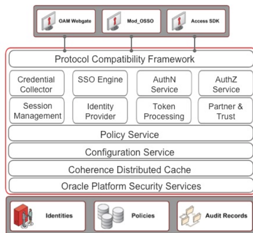
Figure 15: Oracle Access Manager's Architecture
