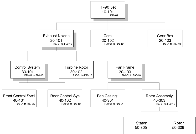
Figure 14-2 Bill of Material for F-90 Jet for Unit Number F90-01
