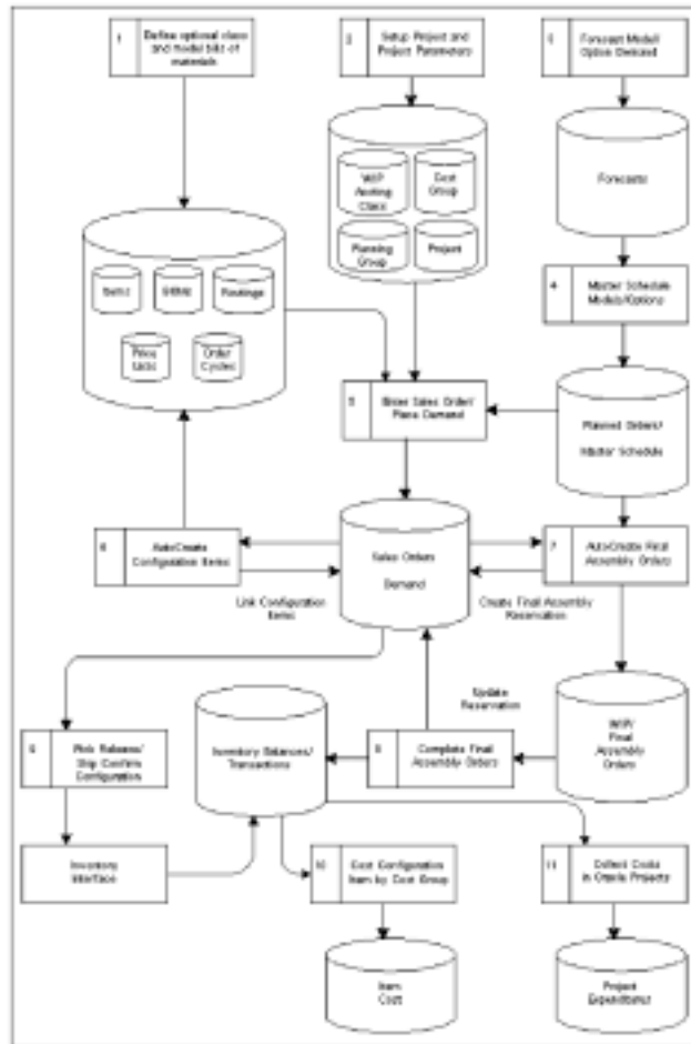
Figure 11-1 illustrates the steps for an ATO/PTO process.
