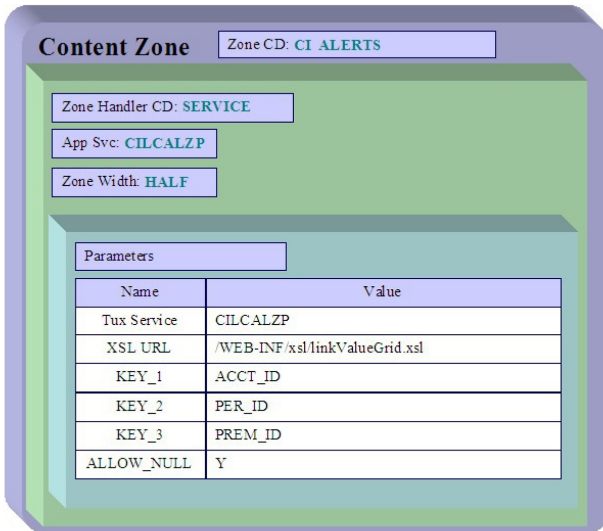
Example Metadata for Service Zone Type
