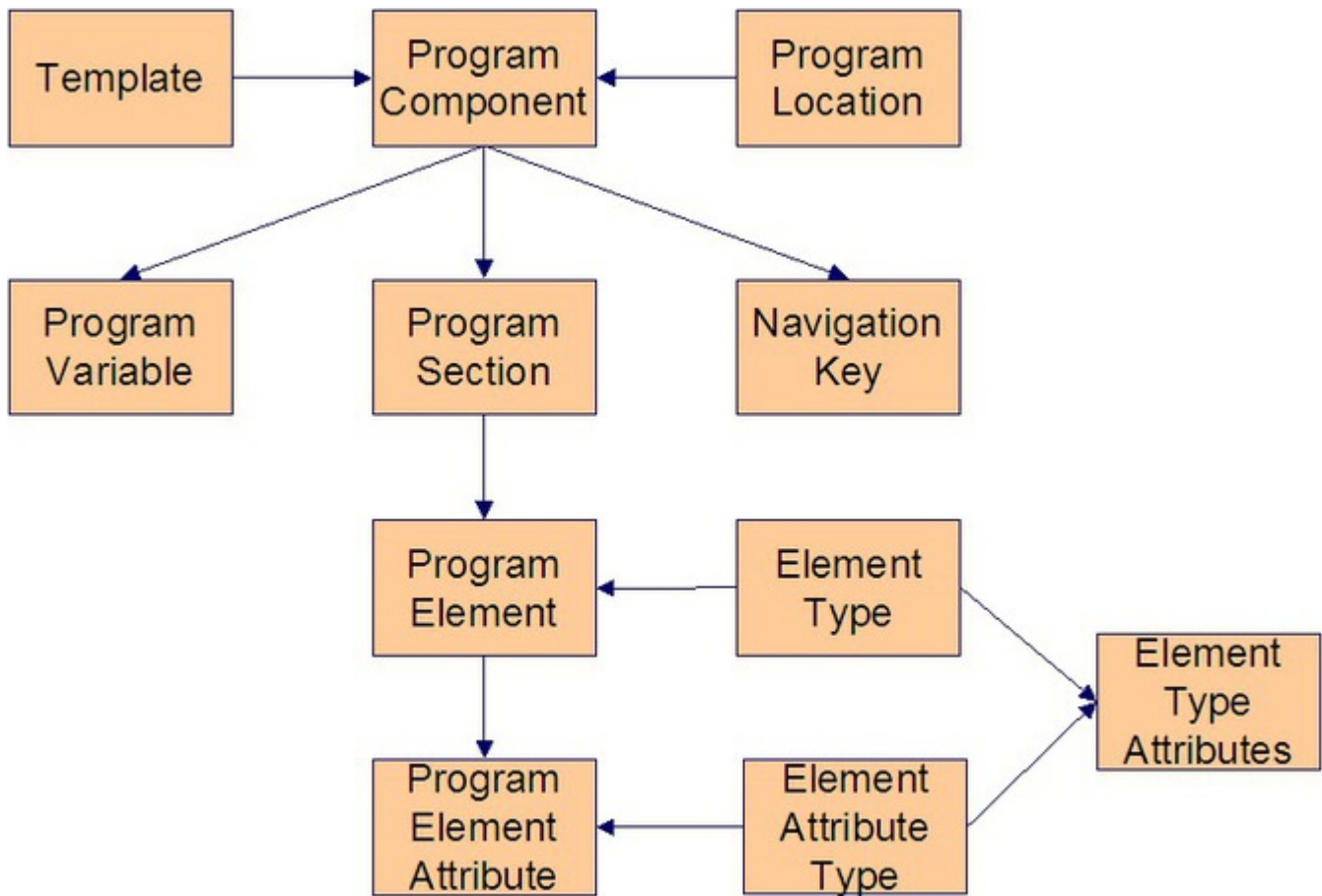
Generated User Interface Program Component Meta-data ERD
