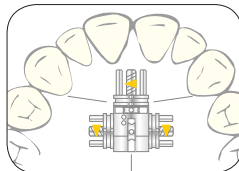
SC2530 Vector 720 expansion screws W17 x H3.6 x L15.7 mm frontal expansion 5.5mm, transversal expansion 7mm
