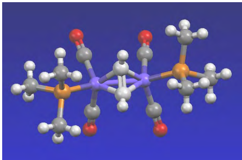
\text{Co}_2[\mu\text{-(HC}\equiv\text{CH)](CO)}_4(\text{PMe}_3)_2
