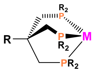
M(\eta^3\text{-tripod}) facial coordinating
