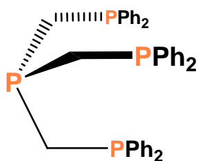
tetraphos-2
