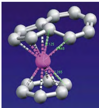
indenyl (-)
