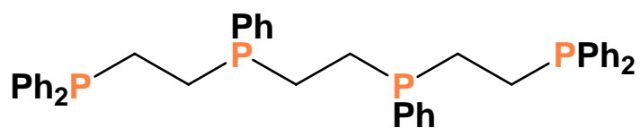
tetraphos-1
