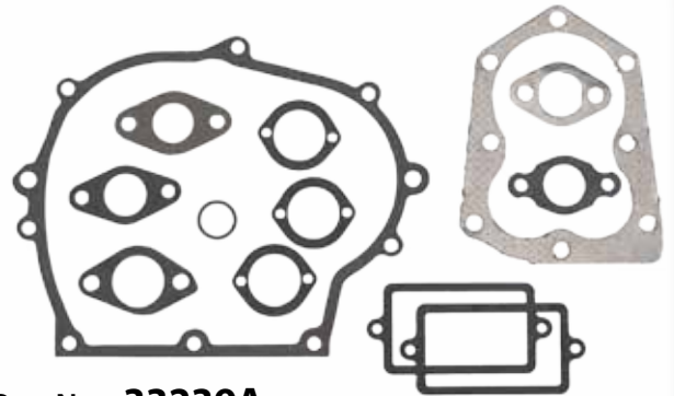
Part No.: 33239A Description: Gasket Set Models Used on: H70, HH70, HSK70, V70, VH70
