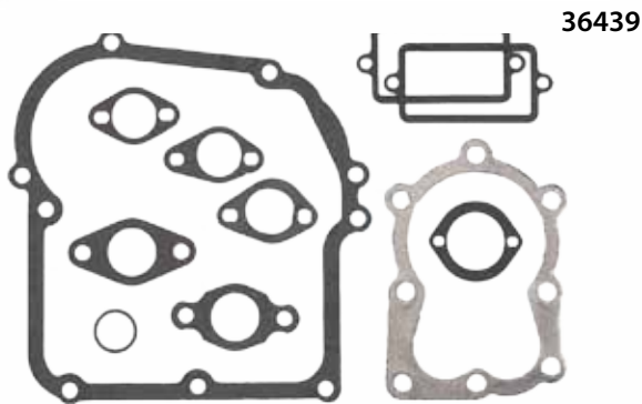
Part No.: 36439 Description: Gasket Set Models Used on: H, HSK40, HT35
