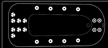
20 JETS (for single-ended baths) To suit models: 652, 653, 683, 954, 956
