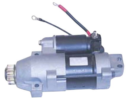
18-6425 STARTER Replaces: 50-804312T1 For: 4 Stroke 75 HP, and 90HP except Verado
