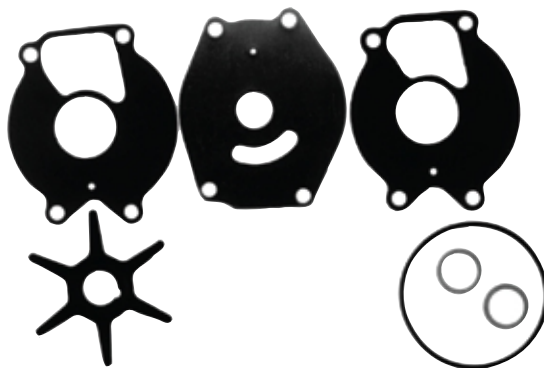
18-3215 IMPELLER REPAIR KIT Replaces: 47-85089T7 — CONTAINS —
