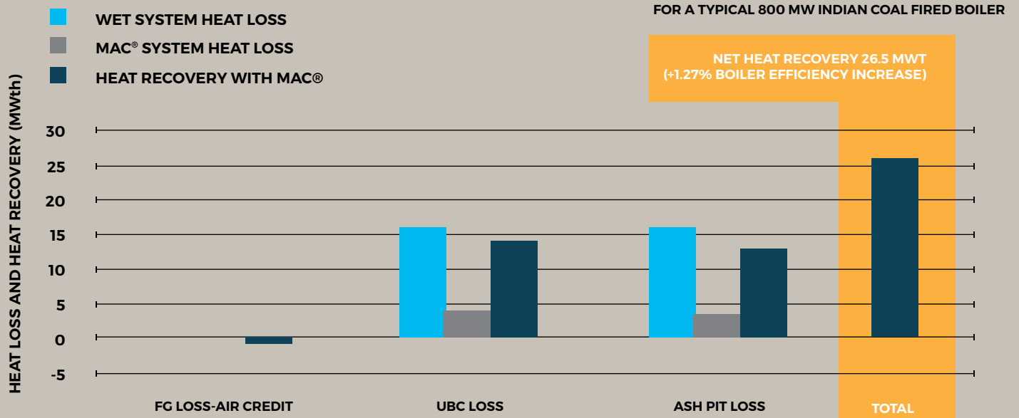
FIGURE 11: TYPICAL EFFICIENCY INCREASE FOR A 800 MW INDIAN COAL FIRED BOILER WITH MAC®/SUPERMAC® SYSTEM
