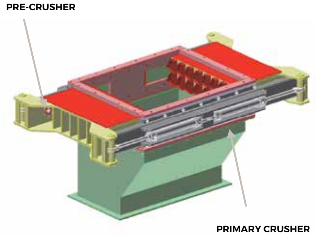
FIG. 3 HYDRAULIC PRE-CRUSHER
