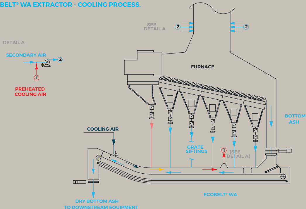
FIGURE 4: ECOBELT® WA EXTRACTOR - COOLING PROCESS.
