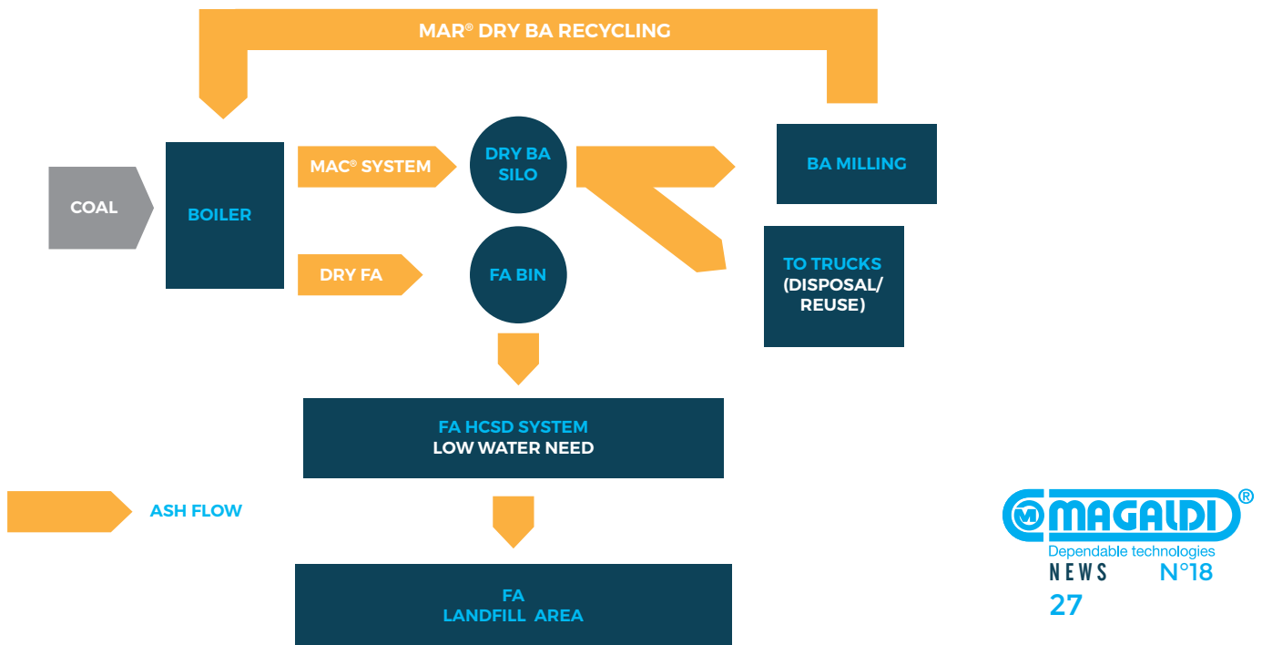
FIGURE 10: SCHEME OF THE MAR® SYSTEM FOR BA CONVERSION INTO FA
