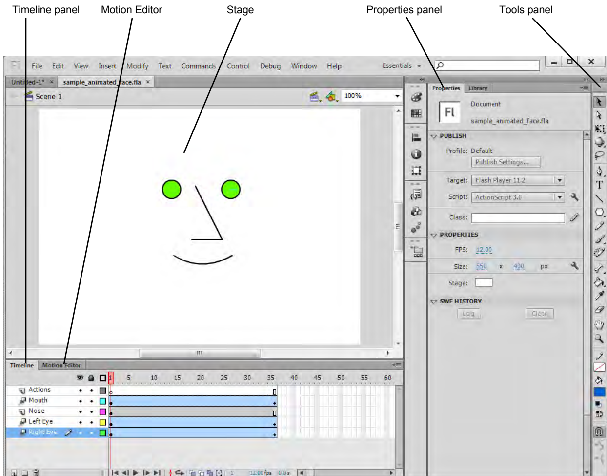
Figure 1 Flash workspace
