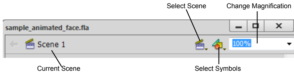
Figure 5 Edit bar
