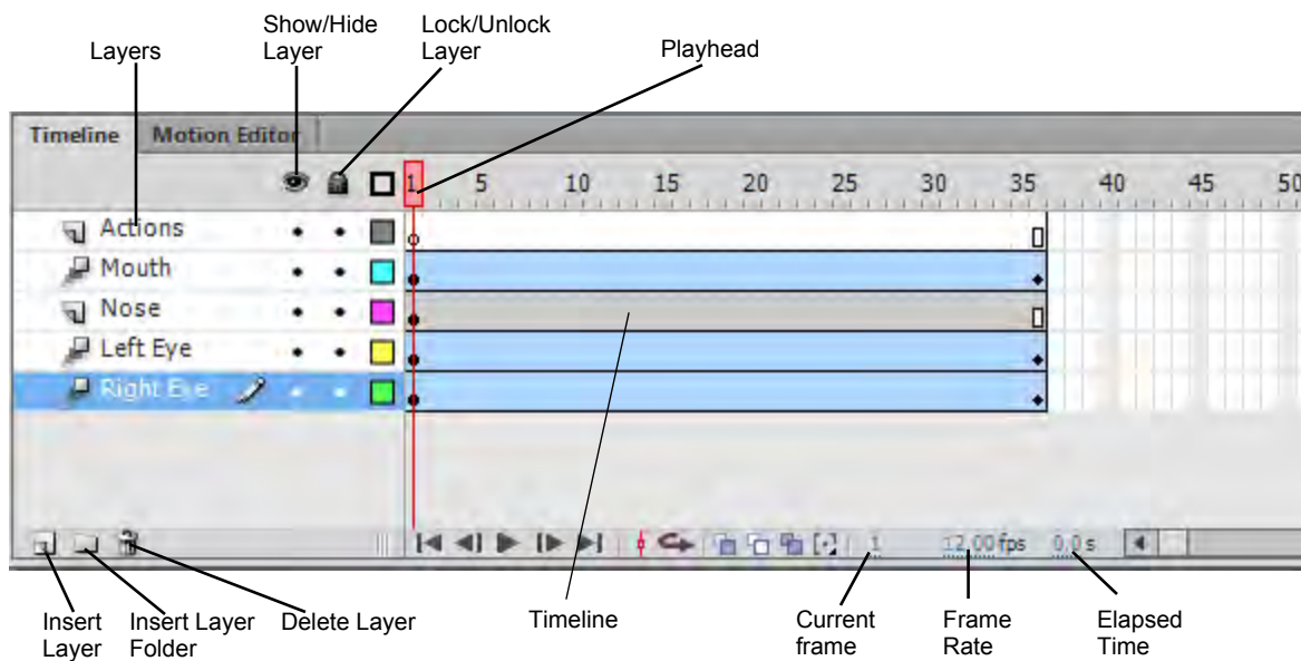
Figure 4 Timeline panel
