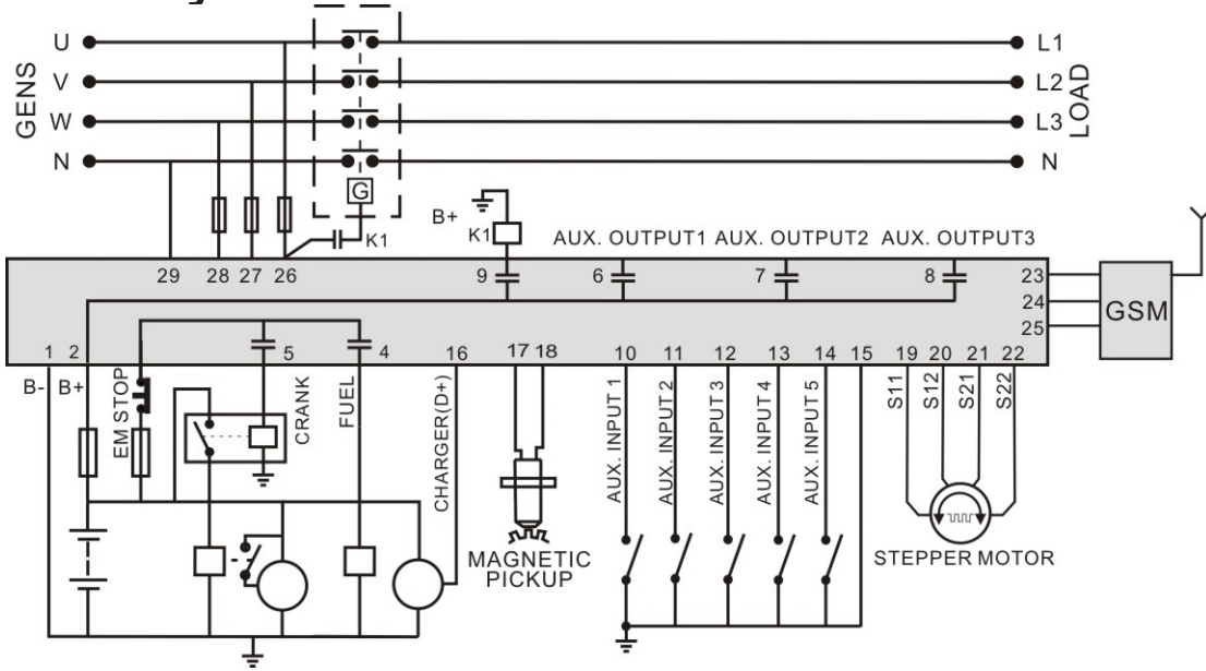
Typical Application Diagram
