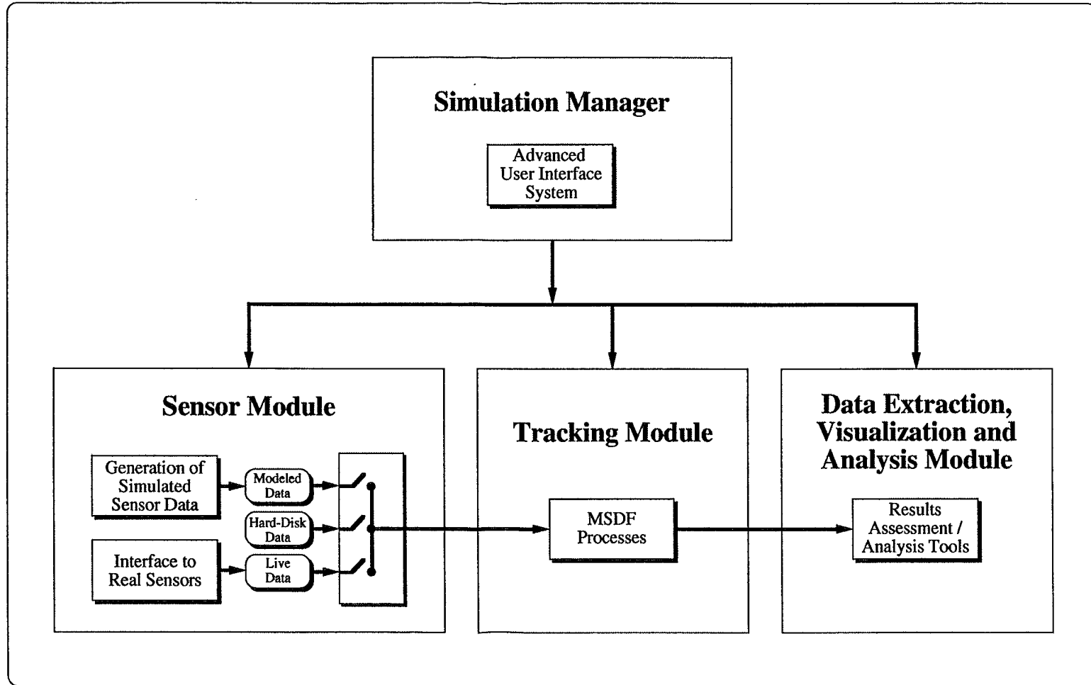
FIGURE 4 - CASE_ATT global structure
