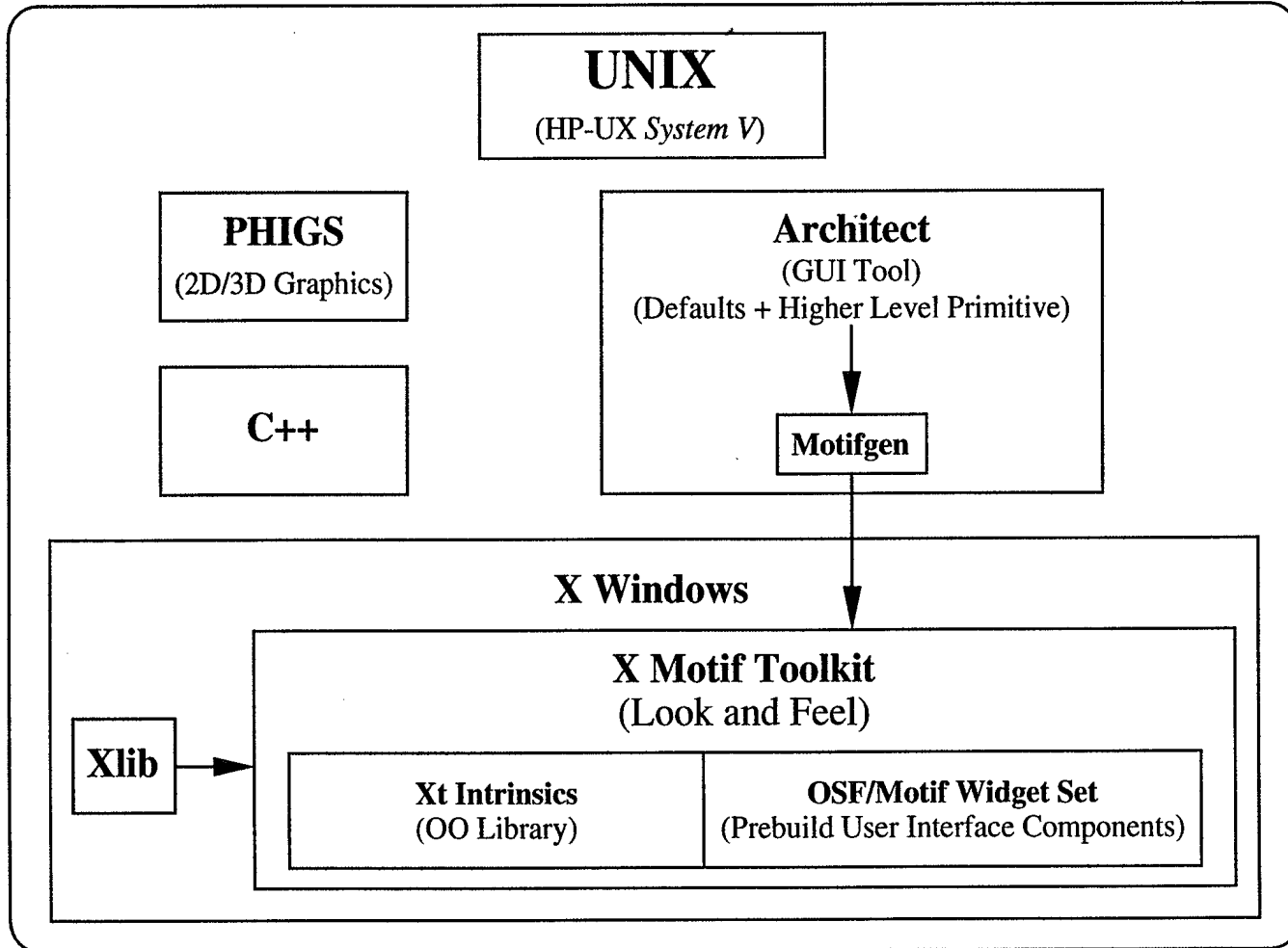
FIGURE 3 - CASE_ATTI software platform
