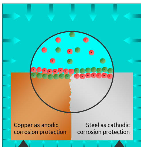
Figure 38: Functional principle
