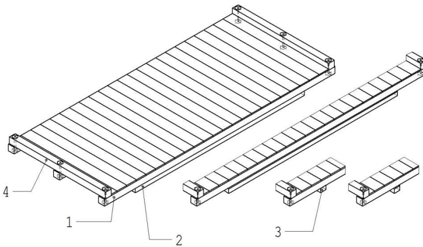
Figure 11: Bottom elements
