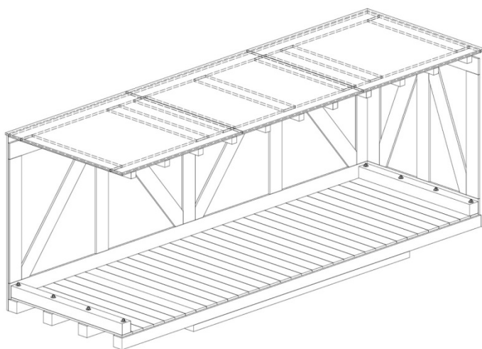
Figure 21: Lid-support members laid on the framework
