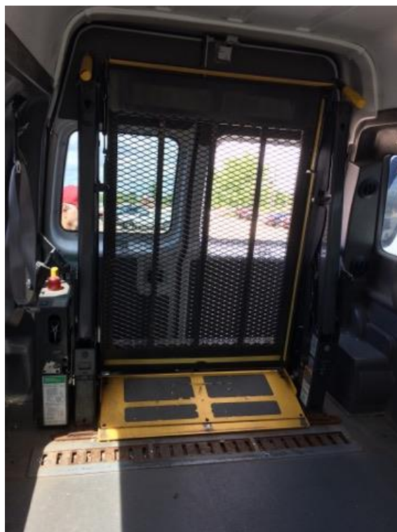
Vehicle Lift: Removed from a Ford E250 Super Duty Van (Tall), Braun Century 2 Series Model: NCL919F1BTB-Z Serial # EA-03078 Mfg Date: 10/15/12, Long Lake
