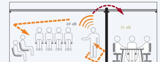
With low absorption ceiling \alpha_w = 0.1 a speaking person generates a sound pressure level of 69 dB.
