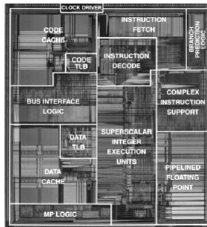
CPU Chip Detail
