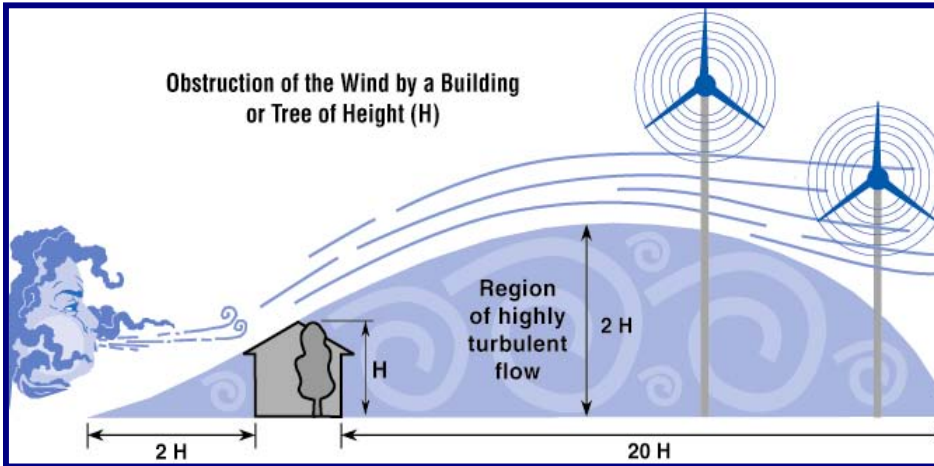
Figure 1: Obstruction Avoidance for Wind Turbines
