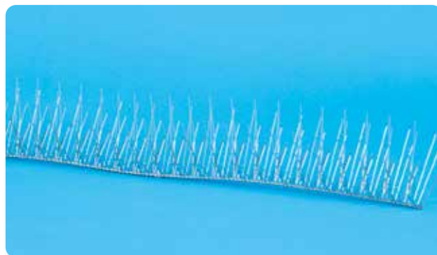
BS364 STARLING AND SPARROW SPIKES STAINLESS STEEL 600mm Strip Dimensions 112mm high x 100mm wide x 600mm long, premium stainless steel spike with 240 points per strip.
