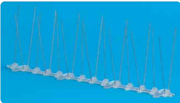
BS272 BIRD-X PIGEON SPIKES NARROW IN STAINLESS STEEL Per Metre 115mm high x 60mm wide between outer tips, base width 40mm
