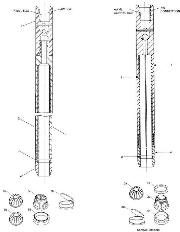
Gambar 5.7 Contoh Split Barrel Sampler
