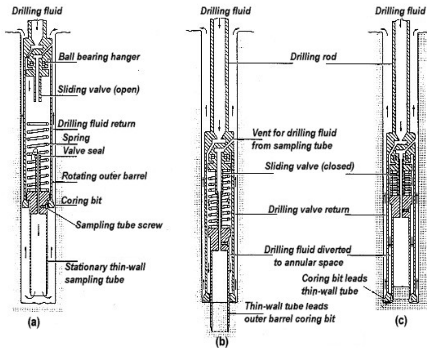
Gambar 5.11 Contoh tabung pitcher (FHWA NHI-01-031)
