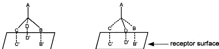
A pair of optical enantiomers showing the different patterns of projection of three functional groups onto a receptor surface
