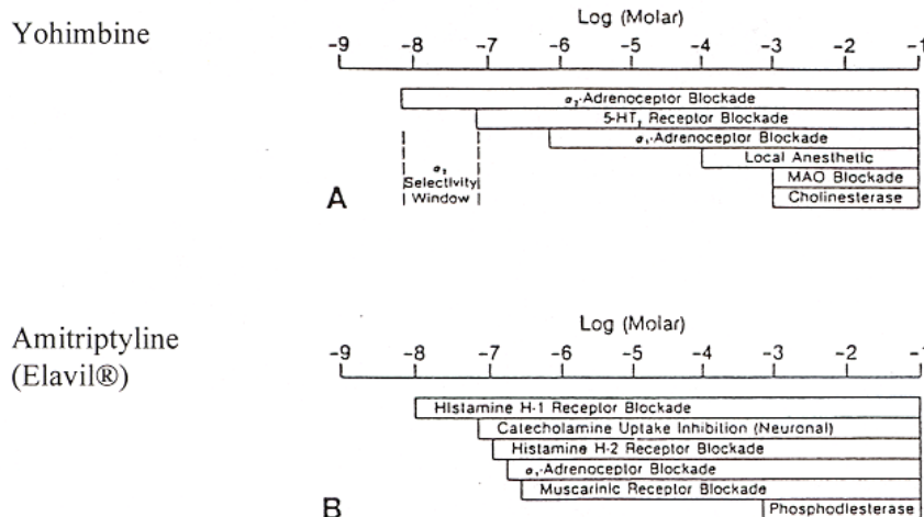
FIG. 1.1 The necessity for a procrustean approach to specificity. A: Yohimbine concentration ranges (on a logarithmic molar scale) necessary for activity for a series of autonomic receptors and functions. B: Similar data for amitriptyline.
