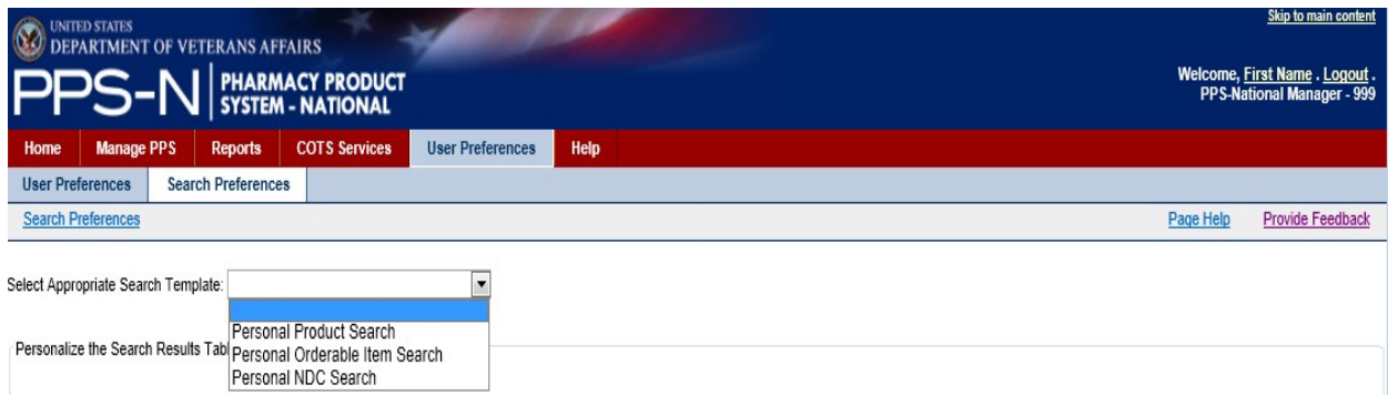
Figure 72: Search Templates
