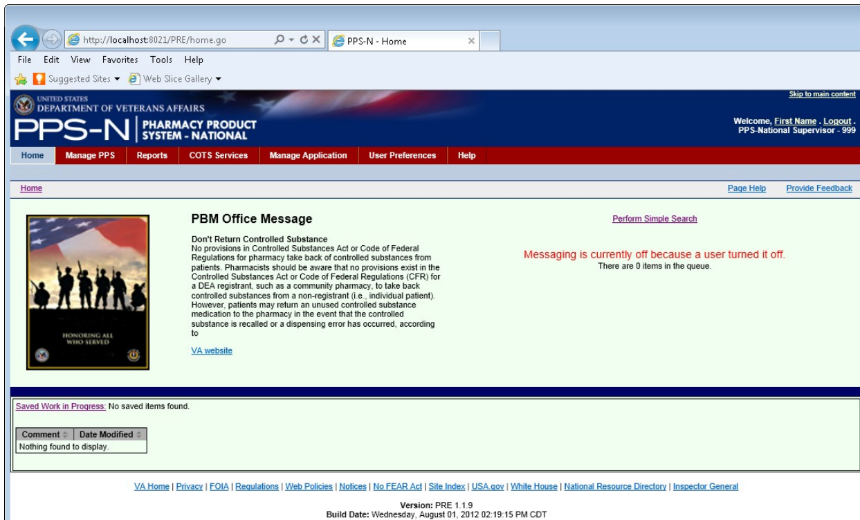
Figure 3: Home Page
