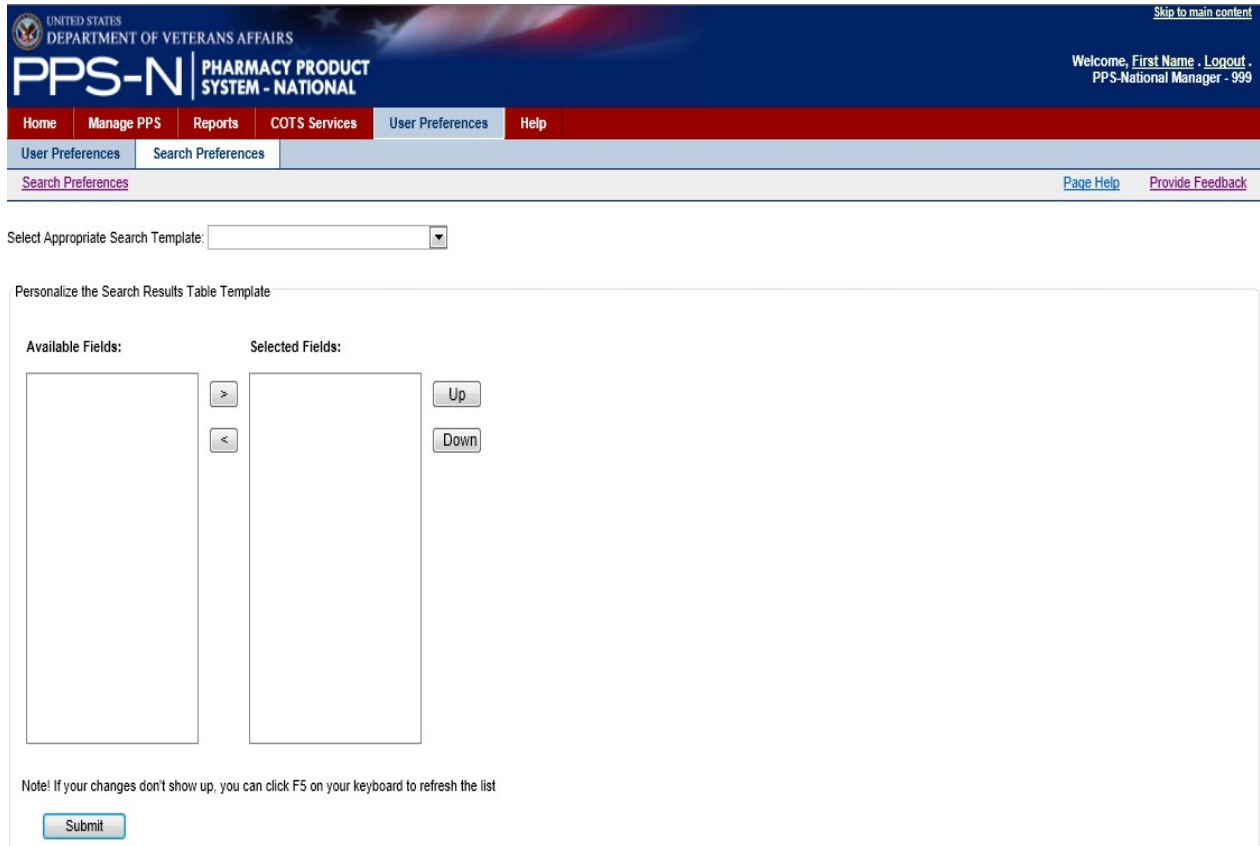
Figure 71: Search Preferences
