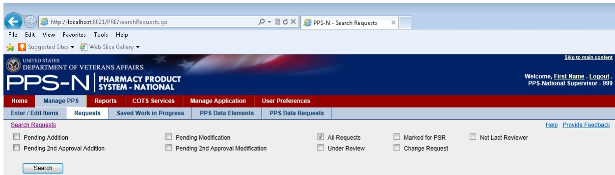
Figure 30: Requests Tab
