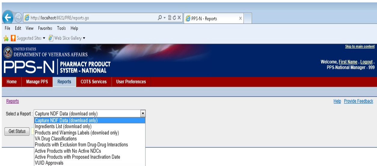
Figure 50: Select Report
