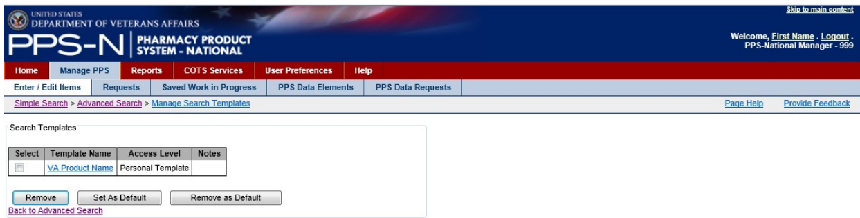
Figure 19: Search Templates
