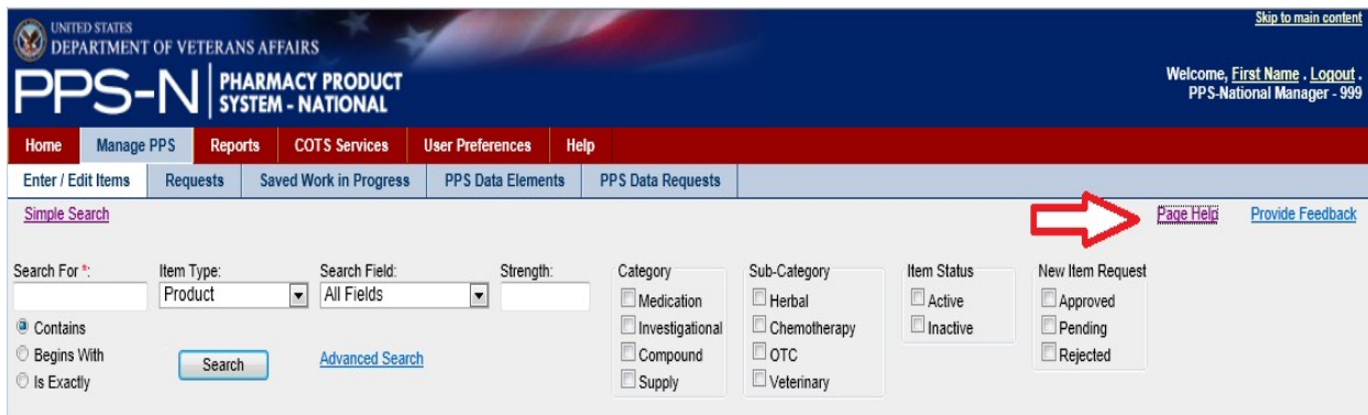
Figure 79: Page Help
