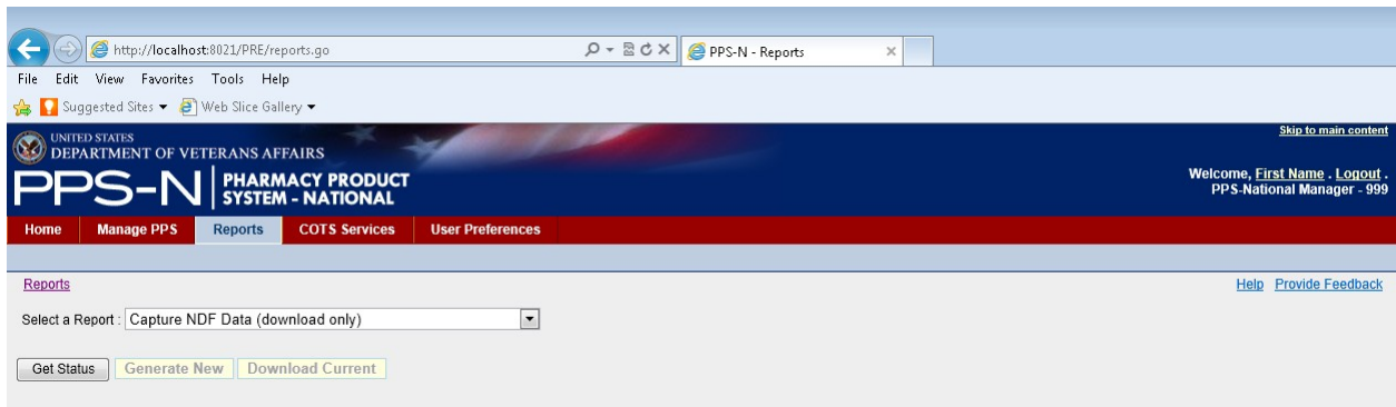
Figure 49: Reports Tab
