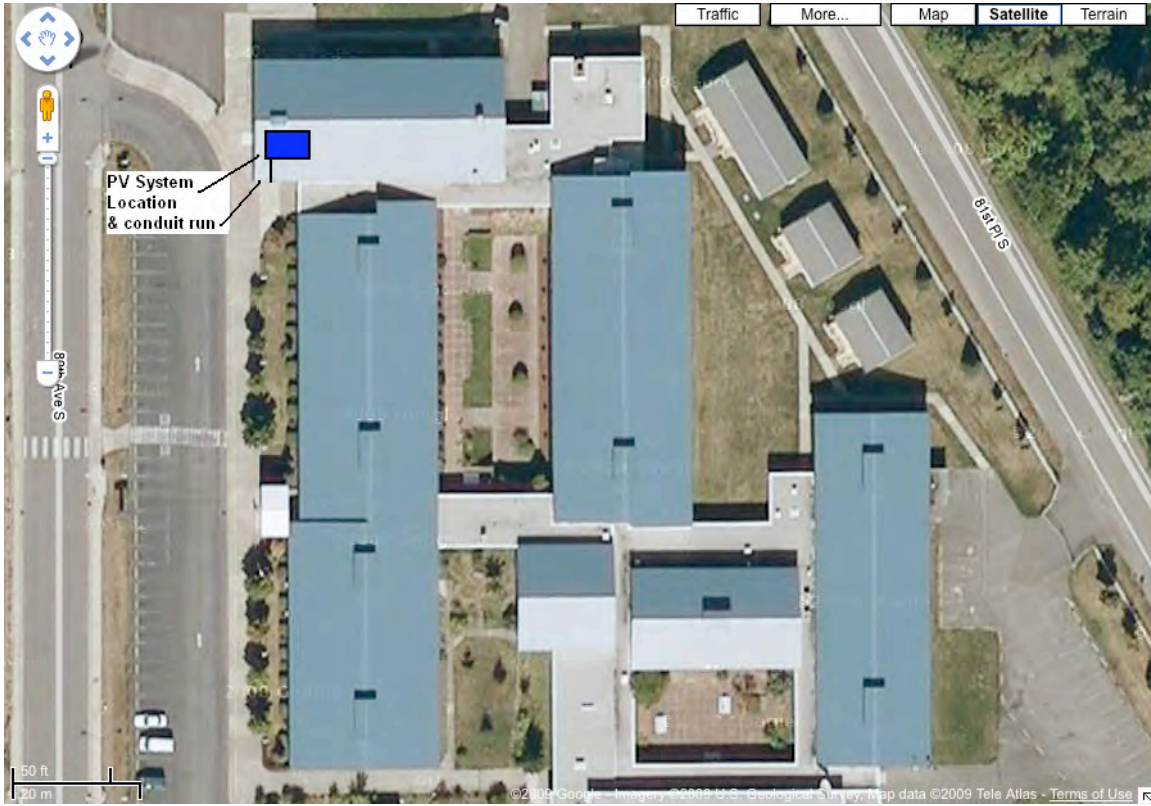
PV array located on the south-facing roof of cafeteria/auditorium building
