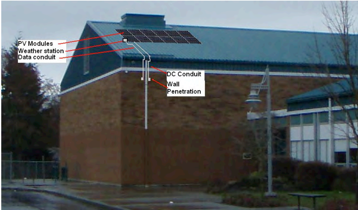
Photo Mock-up of PV array on roof of cafeteria and DC and data conduit running down roof and penetrating wall into backstage area
